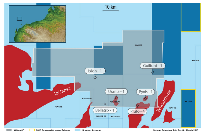
Figure 1. Location map of the Willem 3D seismic survey. The wells within the seismic area are indicated, as are the nearby gas fields and block boundaries. The location of the map with respect to the north-western coast of Australia is shown in the inset.
