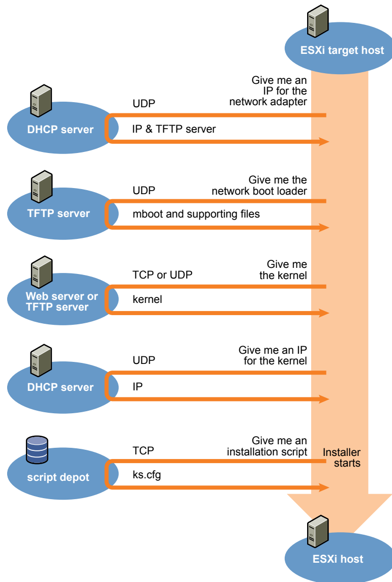
Figure 5-3. Overview of PXE Boot Installation Process
