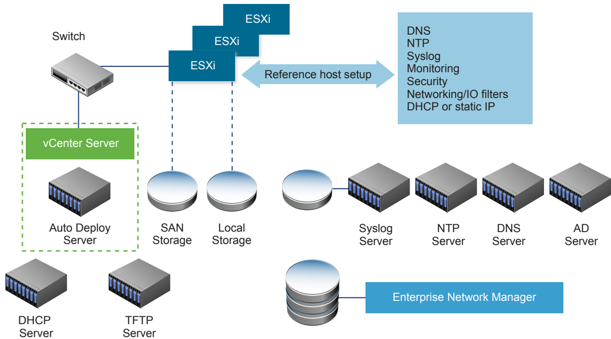
Figure 5-7. vSphere Auto Deploy Reference Host Setup
