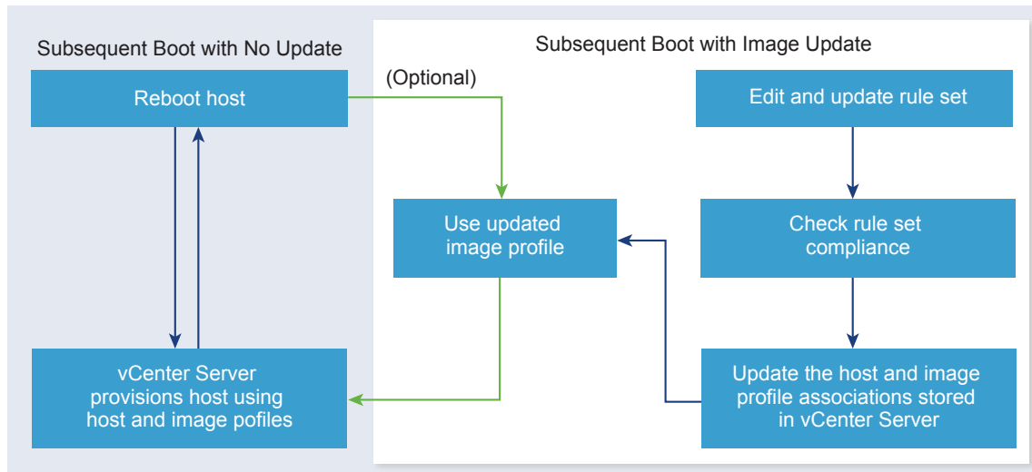
Figure 5-6. vSphere Auto Deploy Installation, Subsequent Boots
