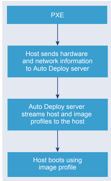
Figure 5-5. vSphere Auto Deploy Installation, First Boot
