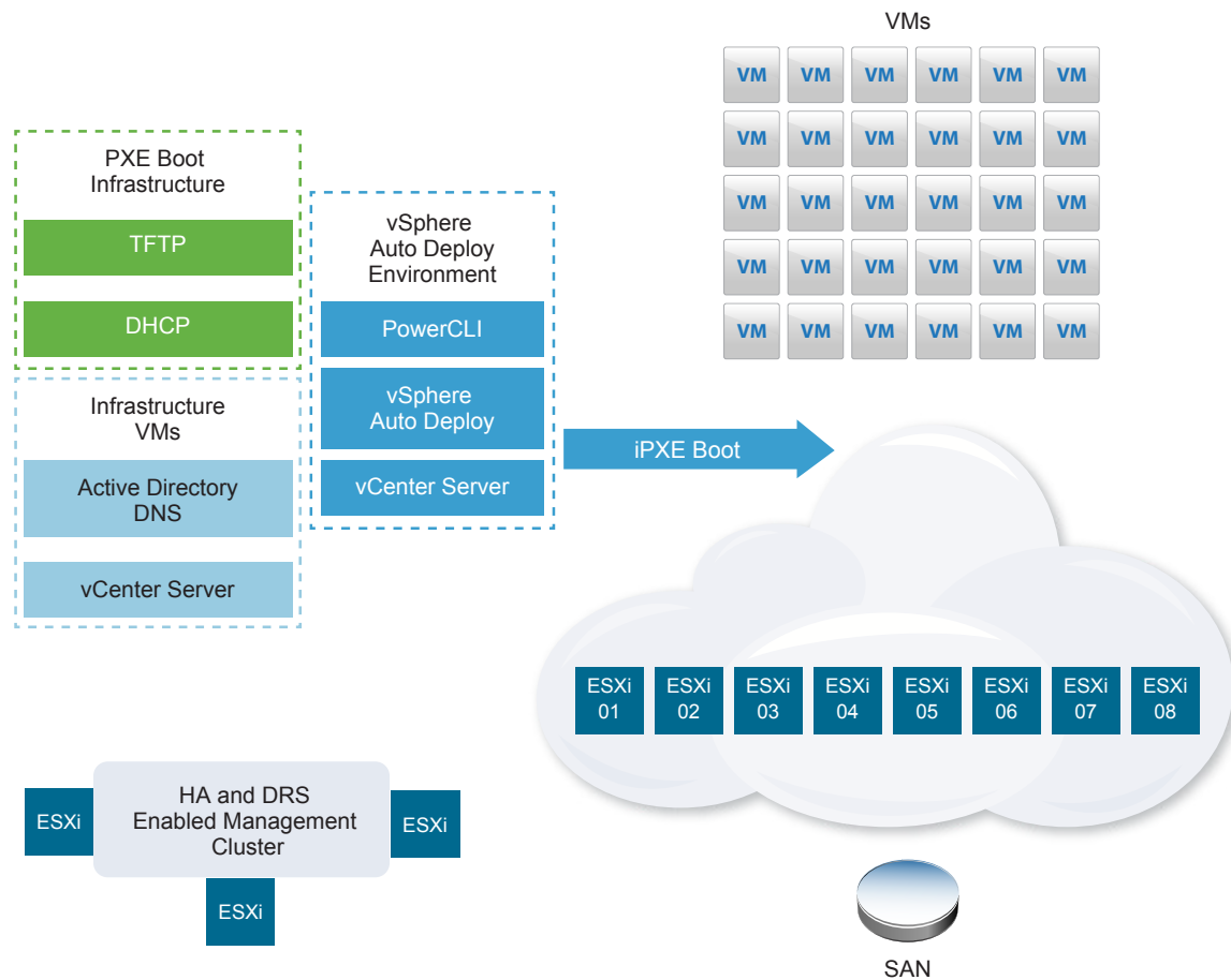
Figure 5-8. Highly Available vSphere Auto Deploy Infrastructure
