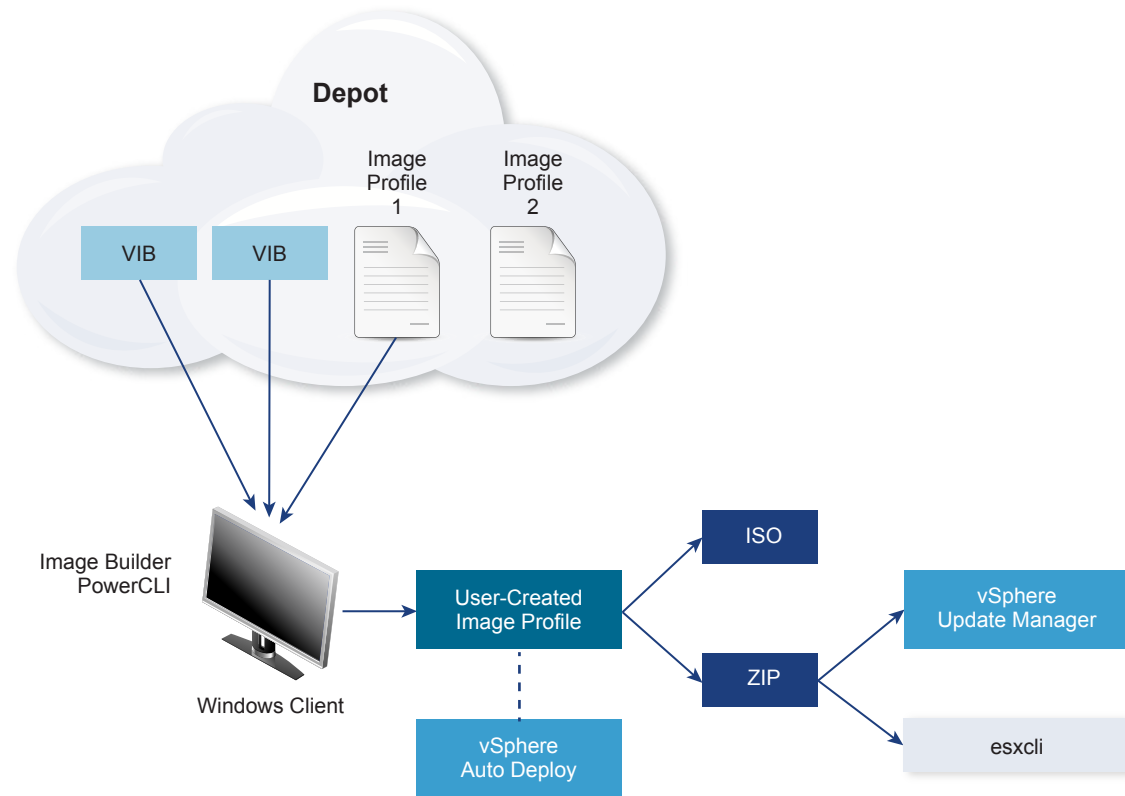
Figure 5-2. Image Builder Architecture
