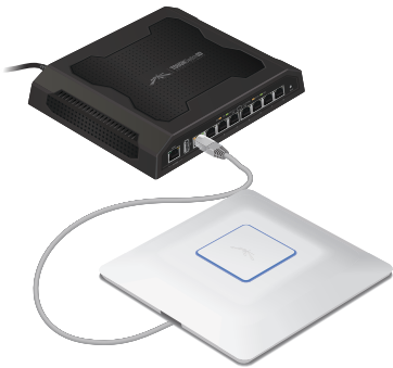
TOUGHSwitch PRO Power Connection Diagram
