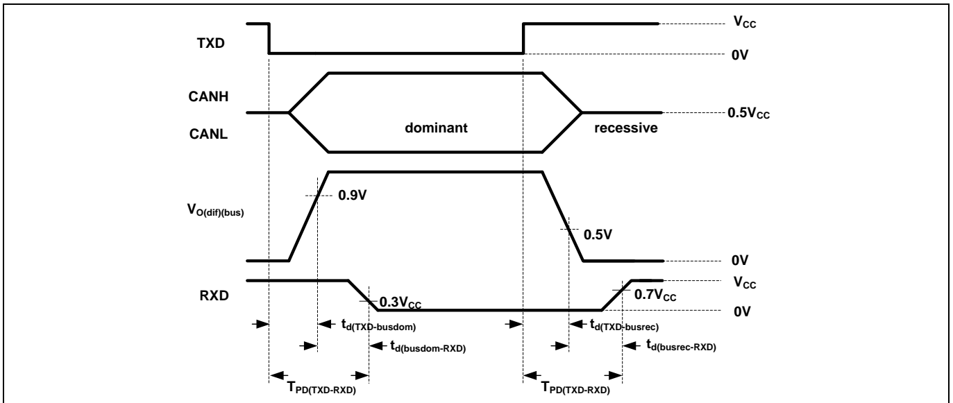
Figure 1. Timing diagram of the CAN transceiver.
