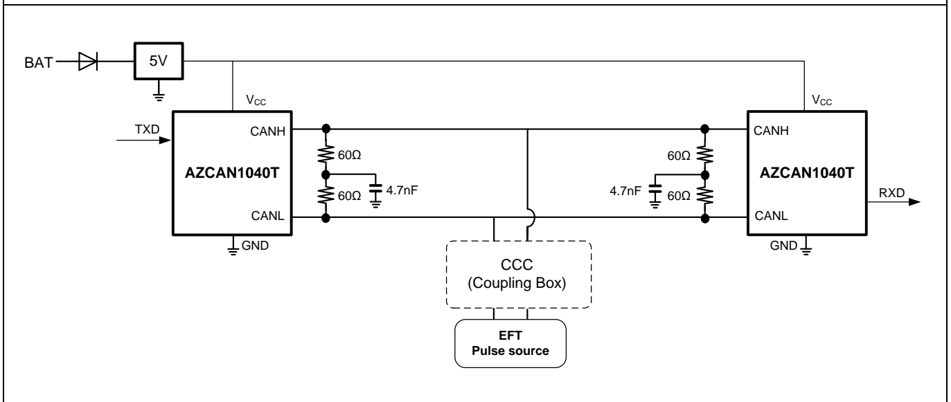
Figure 5. EFT coupling test circuit for AZCAN1040T.
