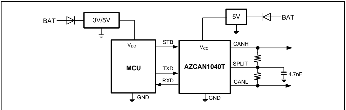
Figure 4. Typical application circuit for AZCAN1040T with 3V/5V MCU.
