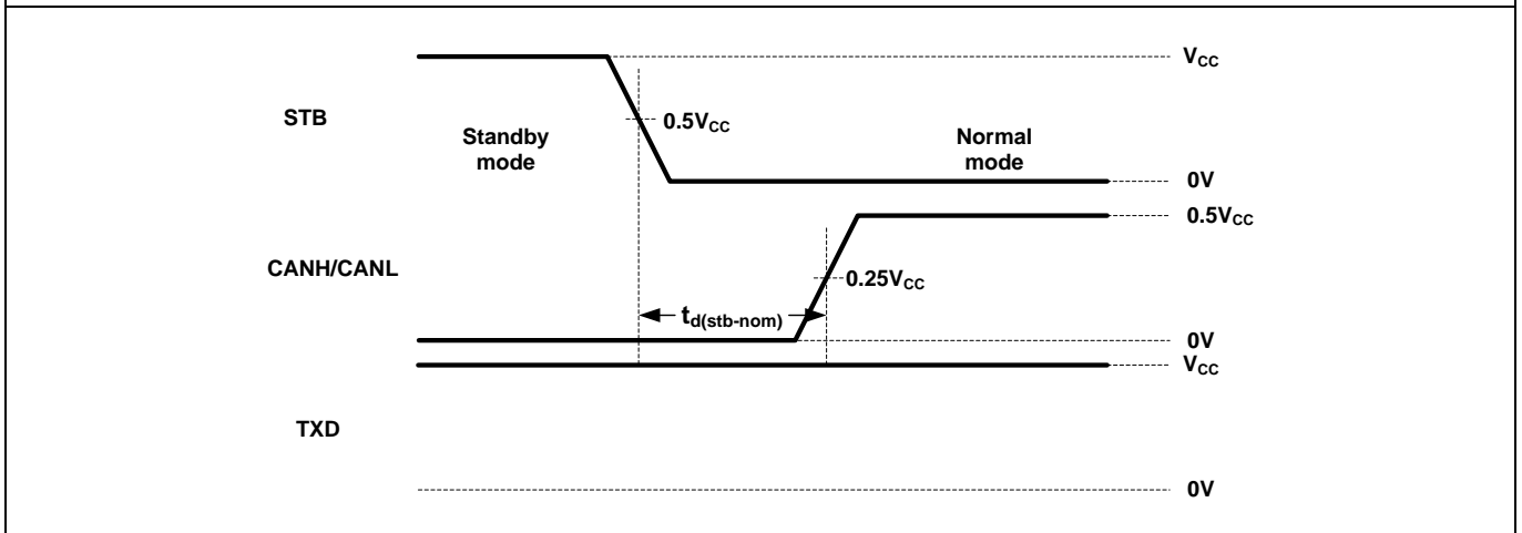
Figure 3. Timing diagram for the delay of the standby to normal mode.
