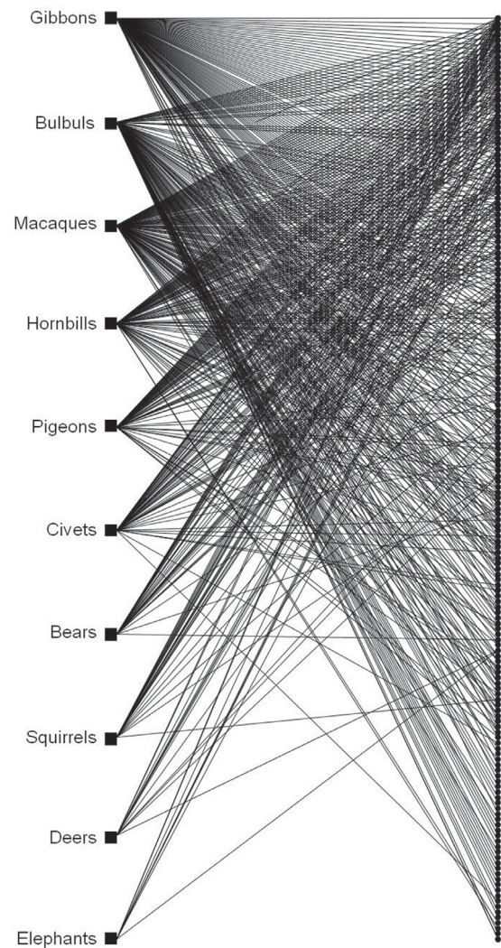
Fig. 1. Bipartite graph depicting a plant-animal mutualistic network involving 10 frugivores (left) and 170 of the plant species (right) they disperse at Khao Yai National Park, Thailand. The list of plant species is based on Kitamura et al. (2002), then the list of frugivores dispersing each species has been completed thanks to data from bin Kassim (1987), Kitamura et al. (2005), Datta & Rawat (2008), Brockelman (2009), McConkey & Brockelman (2011), Albert et al. (2013), Ngoprasert (2012), Khamcha (pers. comm.), Latinne (pers. comm.), Martmoon (pers. comm.).
