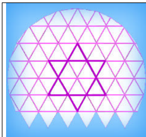
Matrix underlying the Dublin Occult Grid.
