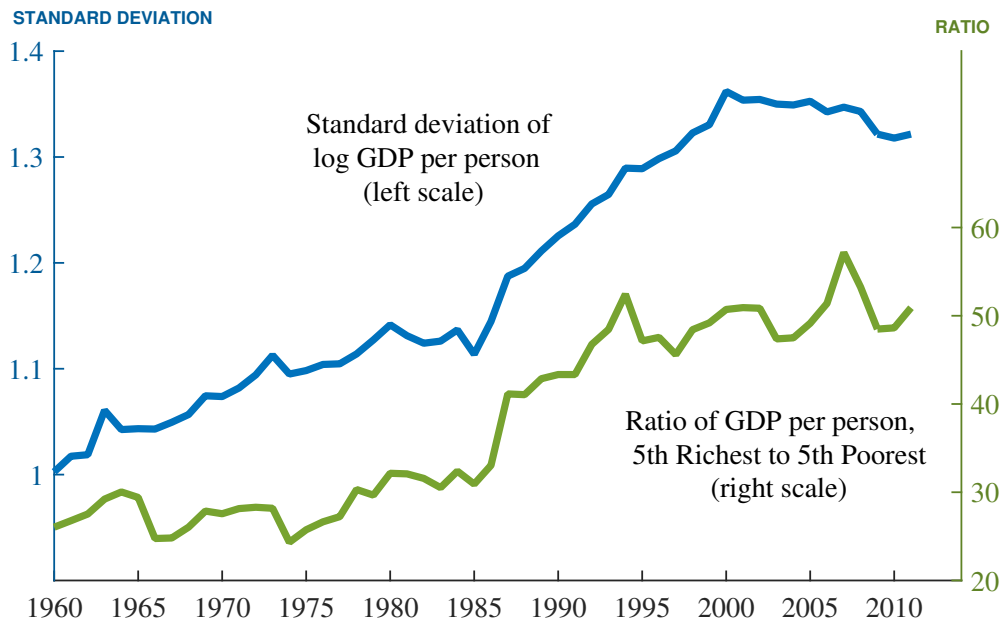
Figure 27: Divergence since 1960
