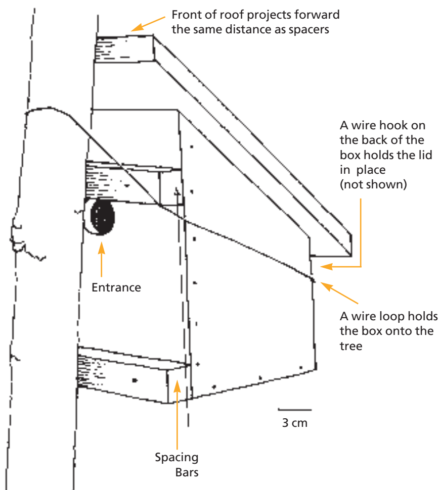
Figure 9 Nest box. Dormouse boxes are like bird boxes, but with the entrance facing the supporting tree or branch. Spacing bars above and below the entrance allow easy access to the entrance hole, which is about 35mm in diameter. The dimensions of the box are not critical. Boxes should be attached using a wire sling, making it easy to take them down for inspection.
