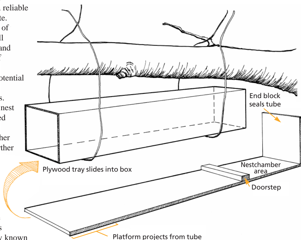
Figure 10 Nest tube. The tube is tied tightly to the underside of a suitable branch with wire. The plywood tray, with attached end stop, slides into the outer tube. Tubes are readily adopted as nest sites by dormice, providing a relatively cheap and easy way of detecting their presence.
