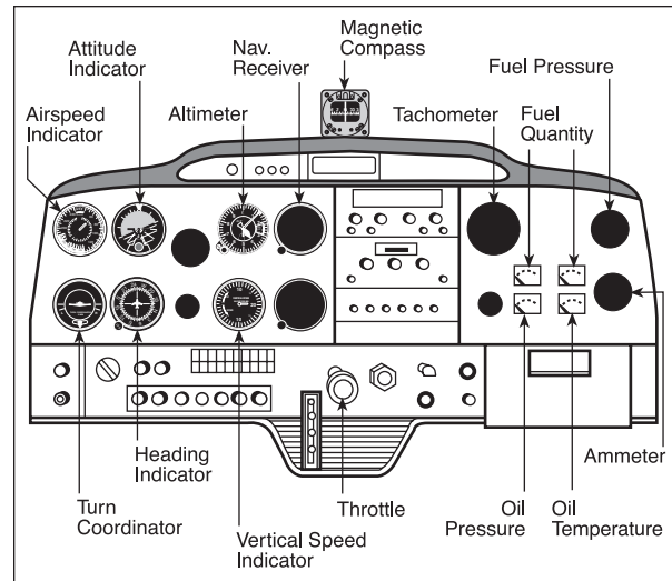
Figure 1-3. Typical “six-pack” of traditional non-digital instruments
