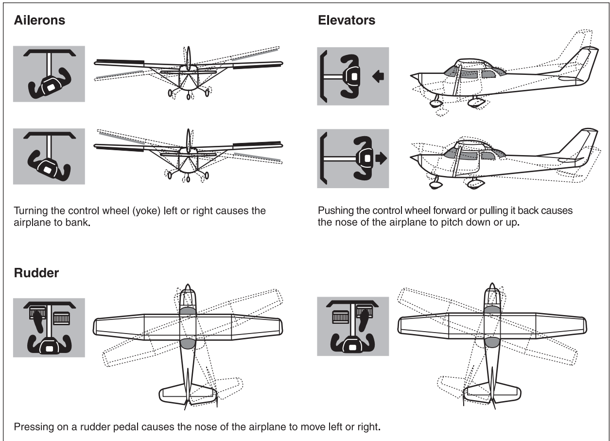
Figure 1-2. Flight controls
