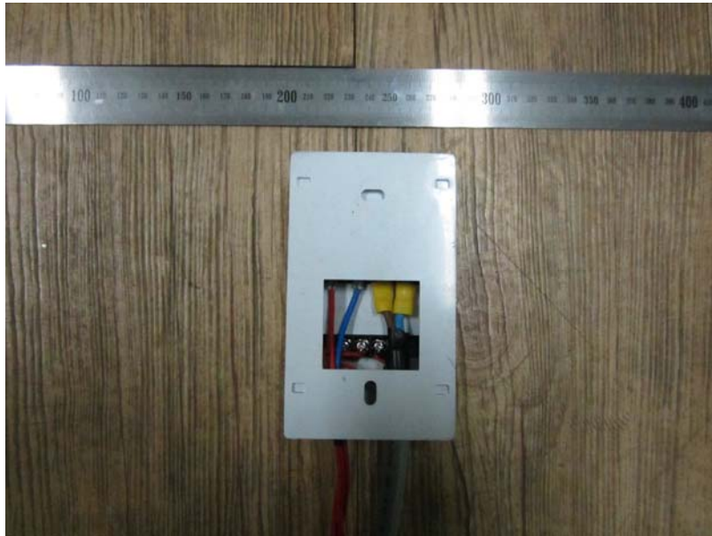
Photo 3 > Rear of controller
