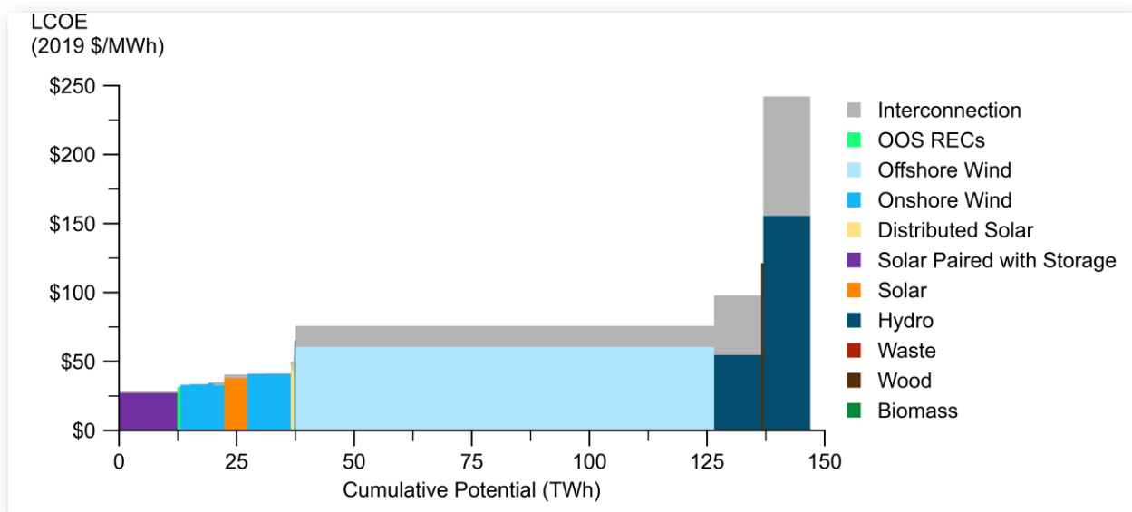
Figure 21. Renewable resource supply curve in 2030
