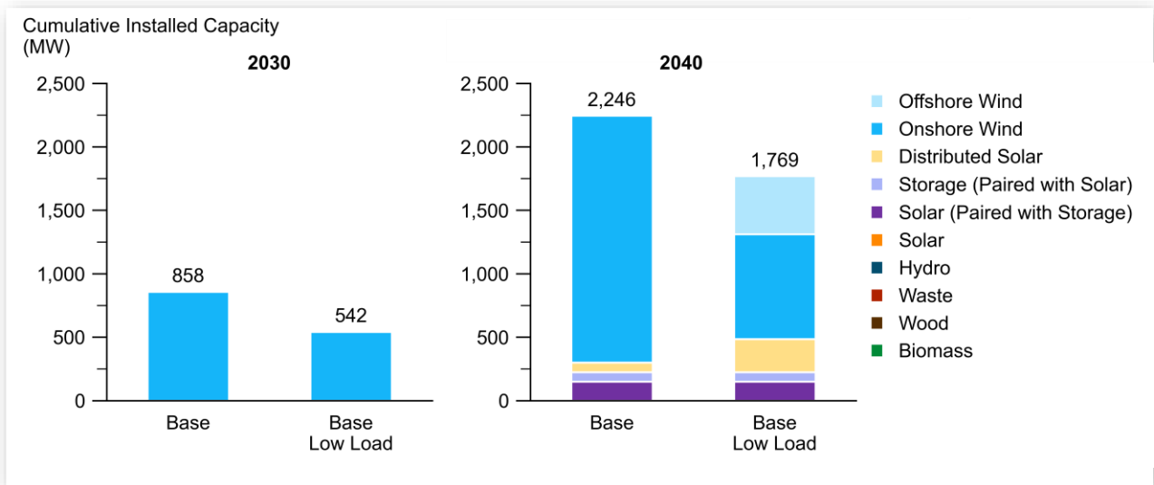
Figure 30. Resource build comparison across Base Case and Base Low Load sensitivity in 2030 and 2040
