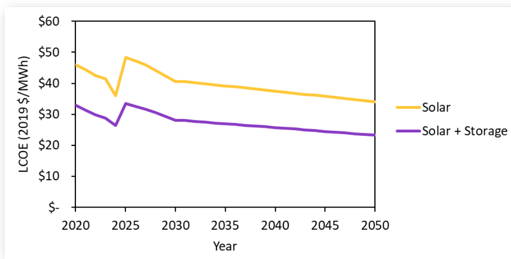
Figure 15. Utility-scale solar costs
