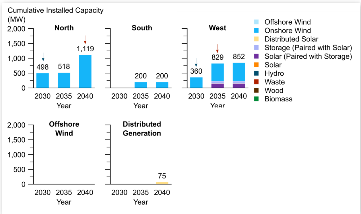
Figure 28. Regional builds in Base Case. The year where the first or second transmission upgrades are needed in each region is indicated by a blue or red arrow, respectively.
