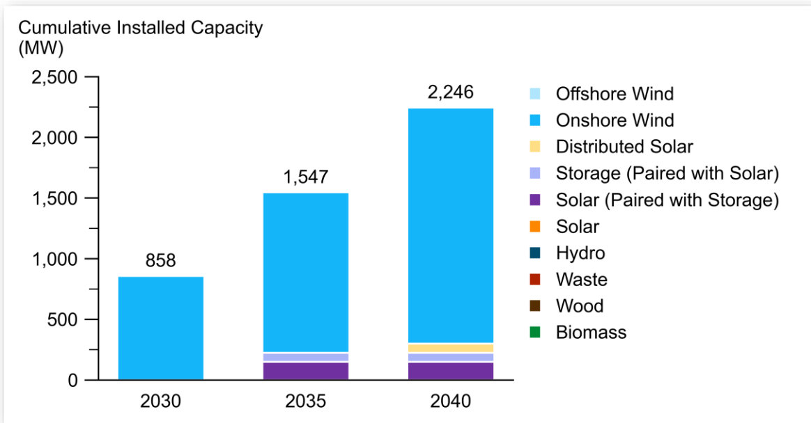
Figure 33. Renewable build in Unconstrained Land Use case
