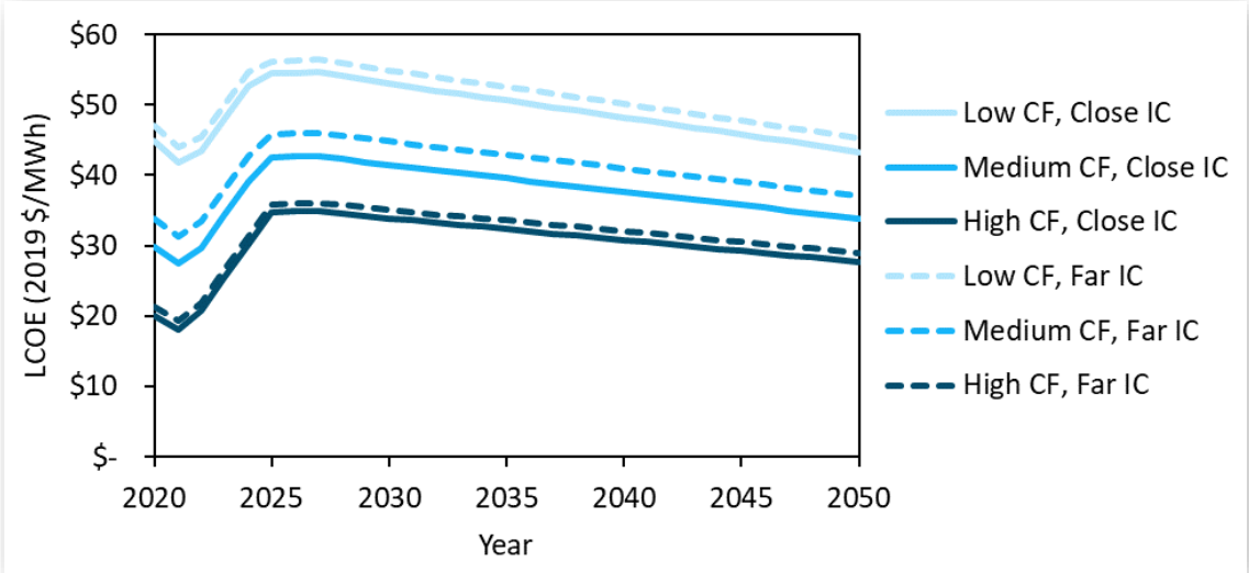
Figure 12. Projected levelized cost of energy (LCOE) as functions of distance to interconnection (IC) and capacity factor (CF) for new onshore wind resources
