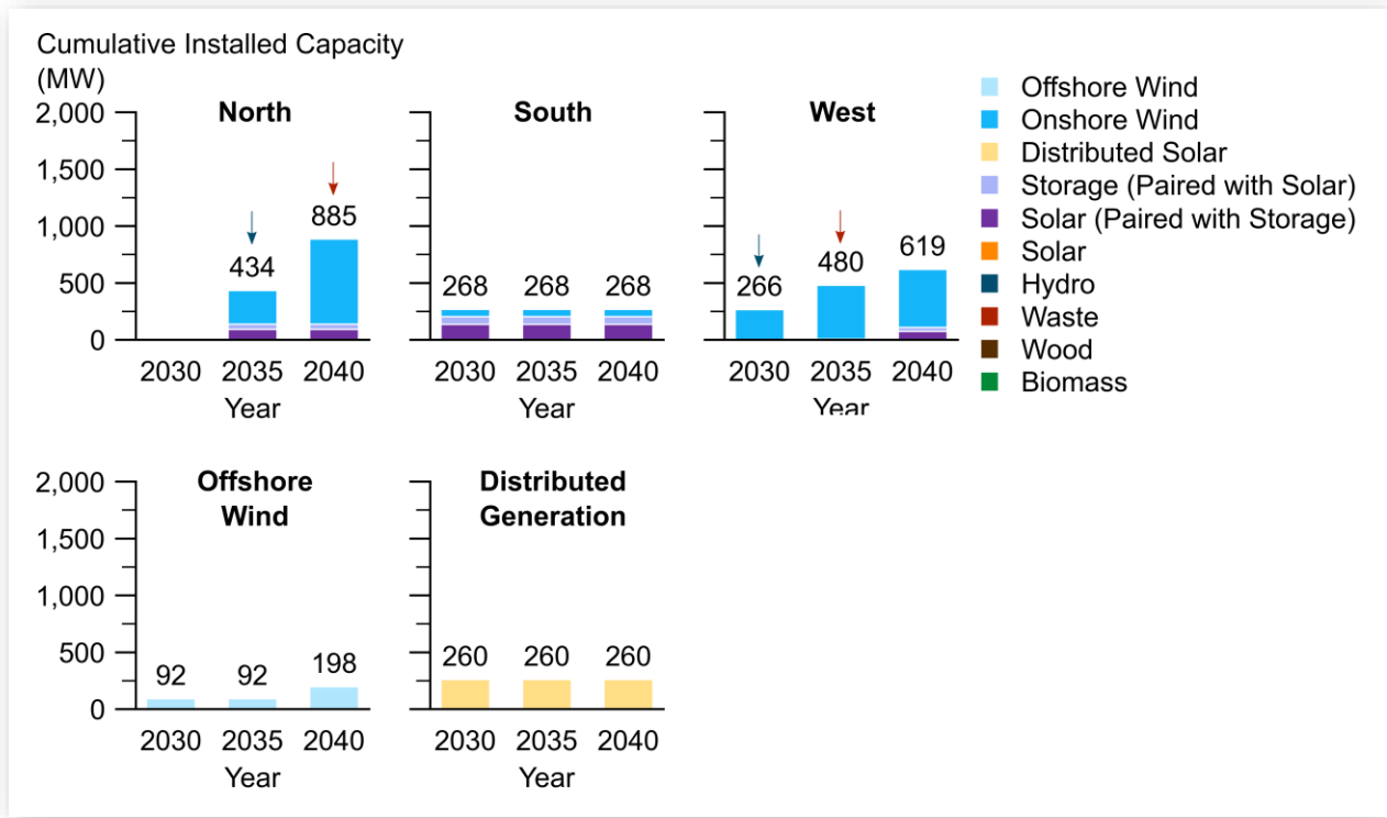
Figure 44. Regional build for Diverse Portfolio case. The year where the first or second transmission upgrades are needed in each region is indicated by a blue or red arrow, respectively.
