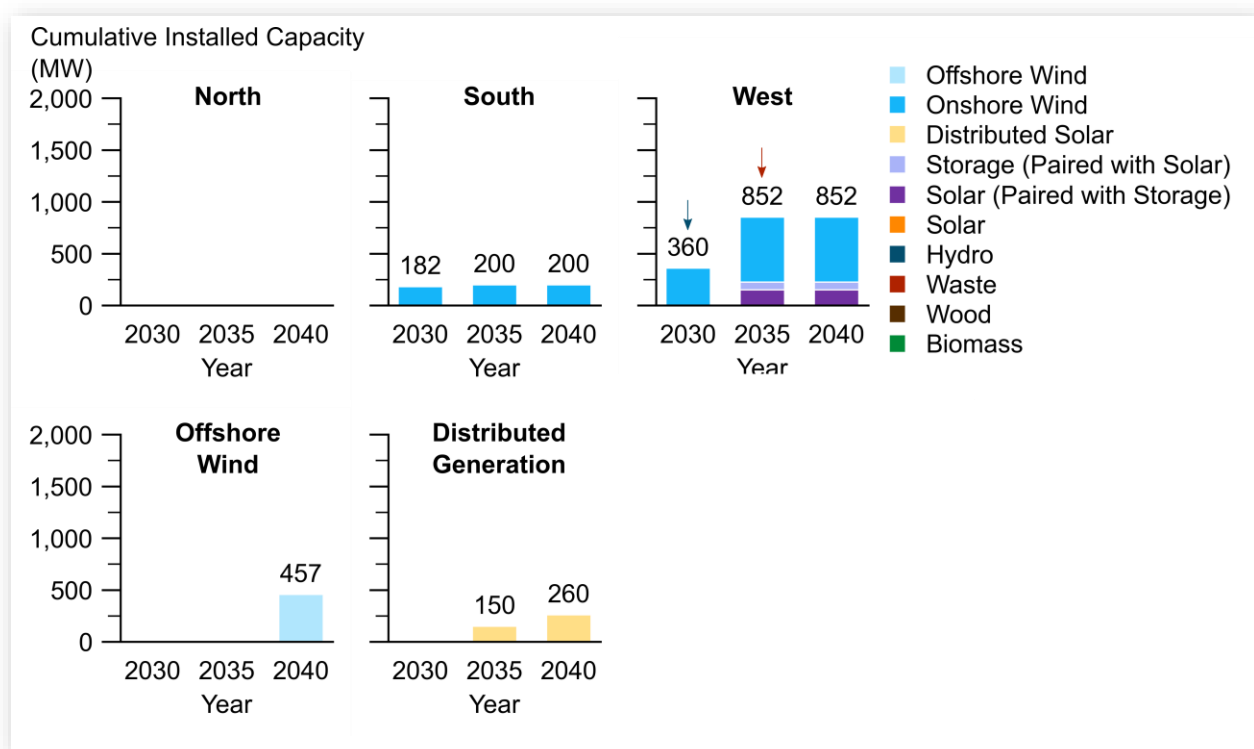
Figure 31. Regional builds for Base Low Load sensitivity. The year where the first or second transmission upgrades are needed in each region is indicated by a blue or red arrow, respectively.
