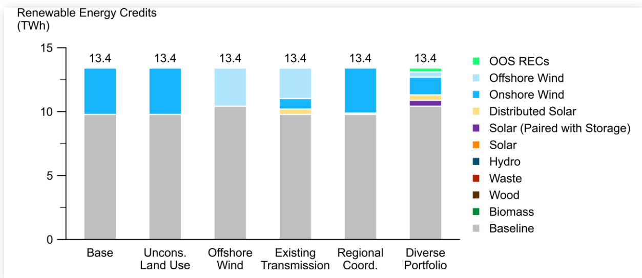
Figure 47. RECs from all sources for all scenarios in 2030.
