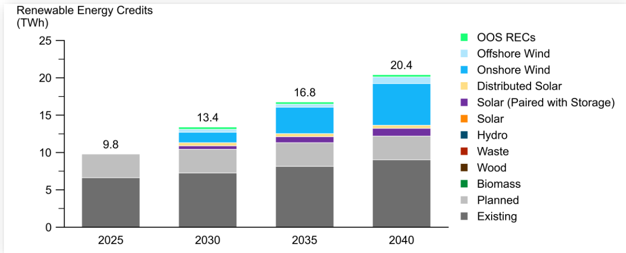
Figure 45. RECs for Diverse Portfolio scenario.
