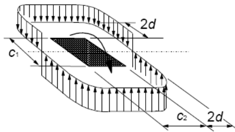
Figure 11.5: Shear distribution due to an unbalanced moment
