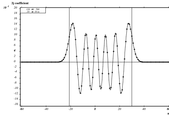
Figure 6.1: Oscillatory behavior of 3j-coefficients.
