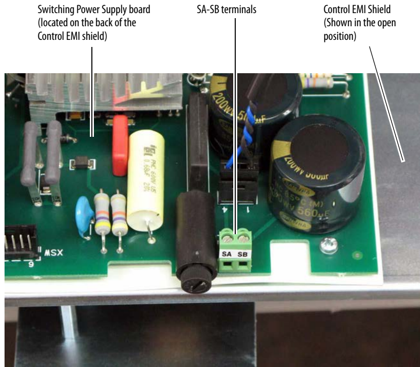
Front of drive shown with top protective cover removed.
