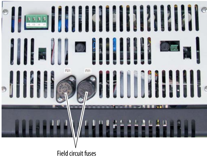
Top View of Drive
