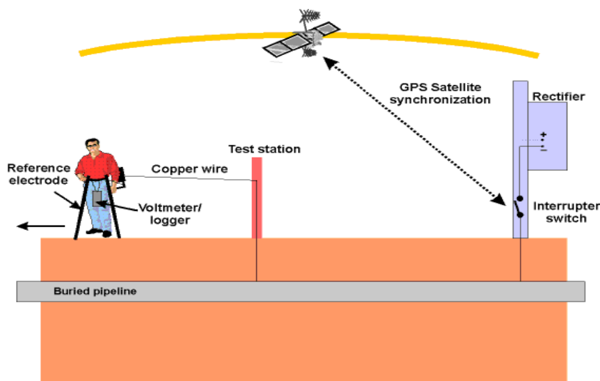
Figure 3.11 – Close-interval pipe-to-soil potential survey (Source: http://www.corrosion-club.com/images/cips1.gif )
