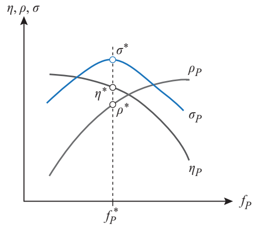
Technology Node: (\sigma^*, \eta^*, \rho^*, f_P^*)
