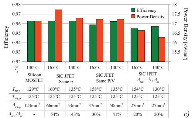
Fig. 13. Basic structure of the power circuit a) of an isolated phase-shift full-bridge DC/DC converter with current doubler rectifier; b) converter prototype optimized with respect to power density (specifications: V_i=400\text{V} , V_o=48\text{V} \dots 54\text{V} , P_o=5\text{kW} , power density \rho=9\text{kW}/\text{dm}^3/147\text{W}/\text{in}^3 ; for further details see [28]); c) efficiency and power density in case Si superjunction MOSFETs (STY112N65M5) or 500V SiC JFETs (SiCED) are employed for realizing the power transistors S_1 - S_4 . Two different junction temperature limits, i.e. T_{j,max}=140^\circ\text{C} and 165^\circ\text{C} are considered for the SiC devices and the chip area is scaled such that an equal efficiency or equal power density is achieved. Furthermore, the properties for an overall die area of the SiC JFETs of A_{SiC}=1/5A_{Si} is shown ( T_{HS,S} denotes the heatsink temperature of the active switches, T_{HS,D} is the temperature of the separate heatsink of the output diodes). The power density values are calculated based on a converter volume determined by summation of the individual component volumes. Accordingly, lower values would result for a practical realization due to not matching geometrical shapes of the components and remaining spaces in between the components.
