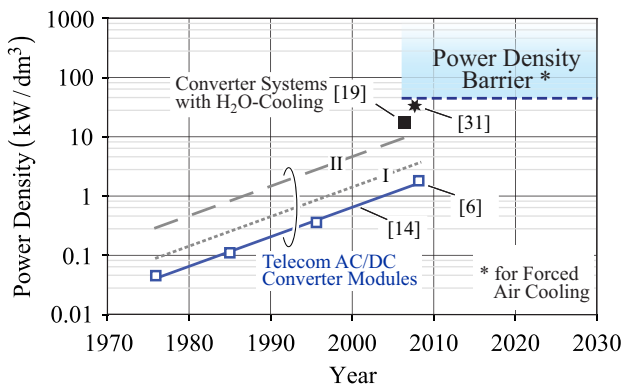
Fig. 19. Improvement of the power density of commercial single-phase telecom AC/DC converter modules (comprising two converter stages, i.e. a PFC rectifier and a DC/DC converter) over the past decades according to [14] and [6]. The increase in power density by a factor of 10 every 20 years has been achieved by changing from natural convection to forced air cooling and by increasing the converter switching frequency. Curve I characterizes the power density trend of the individual converter stages, i.e. of the PFC rectifier or DC/DC converter stage; II indicates the performance development of research demonstrator systems which are translated into commercial products typically within 10 years. Furthermore shown: Power Density Barrier of forced air cooled converter systems as calculated in [17] and local power density of a water cooled non-isolated bi-directional automotive DC/DC converter (Fig.21a) and of an unidirectional three-phase/level PFC rectifier system (Fig.18).
