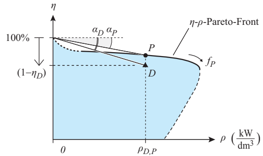
Fig. 8. \eta - \rho -Pareto Front resulting for optimization of a power converter concerning efficiency \eta and power density \rho , i.e. (w_\eta \eta + w_\rho \rho) \Rightarrow \text{Max} . In case of a lower weighting w_\eta of the efficiency, higher switching losses are tolerated and/or higher frequencies f_P are selected by the optimization algorithm resulting in higher power densities. In order to consider the inherent trade-off between efficiency and power density the performance of a converter system and/or design D should be evaluated based on the ratio \tan \alpha_D = (1 - \eta_D) / \rho_D , where \tan \alpha_P represents the maximum obtainable performance.
