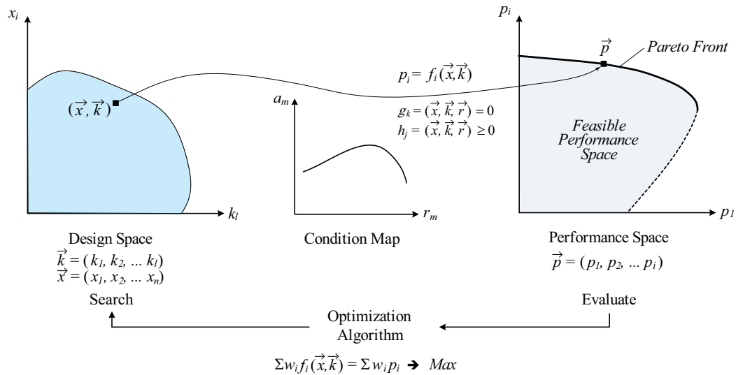
Fig. 4. Abstraction of the design and multi-objective optimization of a power electronics converter as mapping of a multi-dimensional Design Space (or Decision Space) into a multi-dimensional Performance Space (Objective Space). The boundary of the Feasible Performance Space is defined by the Pareto Front which indicates the best possible compromise with respect to different performance indices [14]. In case the whole mission profile of a converter is considered for the optimization, a probability density a_m is assigned to the various operating points, resulting in a multi-dimensional Condition Map [15].
