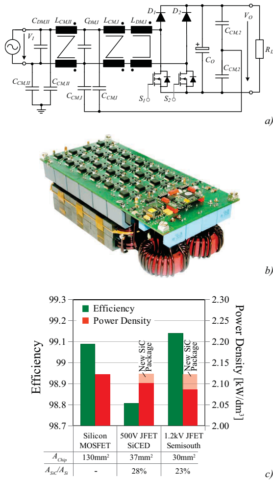
Fig. 16. Basic structure of the power circuit a) of a single-phase bridgeless PFC rectifier with capacitive coupling of the output voltage to ground (capacitors C_{CM,1} and C_{CM,2} , [14]); b) converter prototype optimized with respect to efficiency (specifications: V_I=230V_{rms}\pm 10\% , V_O=365V , P_O=3.2kW , rated power efficiency \eta=99.2\% ; for further details see [14] and [28]); c) efficiency and power density for realizing the power transistors S_1 and S_2 with Si-superjunction MOSFETs (IPP60R099CP) of a normally on 500V SiC JFETs (SiCED) or 1.2kV normally off SiC JFETs (SemiSouth). The power density values are calculated based on a converter volume determined by summation of the individual component volumes. Accordingly, lower values would result for a practical realization of the converter systems due to not matching geometrical shapes of the components and remaining spaces between the components. Furthermore given: chip areas resulting from the efficiency optimization.
