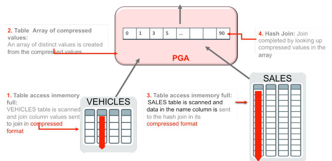
Figure 27. Steps necessary to complete a Hash Join Plan with a Join Group
