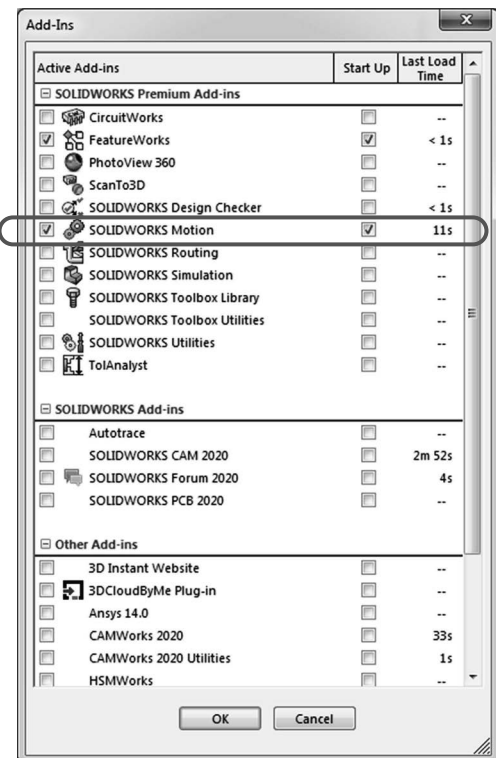
Figure 1-18 The Add-Ins Window
