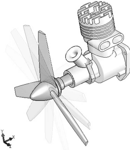
Figure 1-16 Motion Animation
