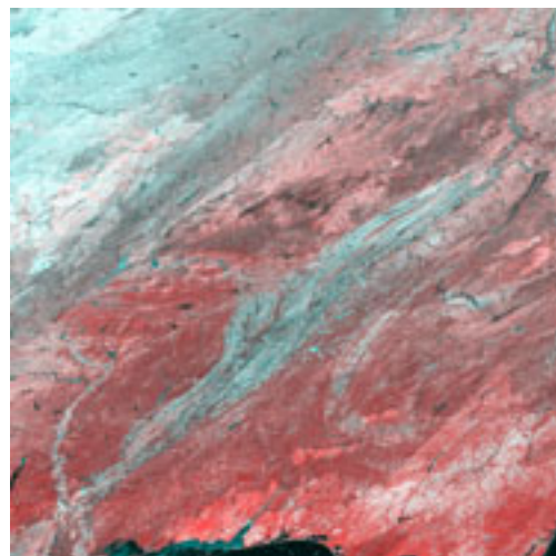
Figure 6. An example of MOD09Q1 surface reflectance product. The corresponding MODIS data were collected in December, 2000 over Alabama, Mississippi and Florida. Product Granule ID: MOD09Q1.A2000337.h10v05.005.2006342044337.hdf.
