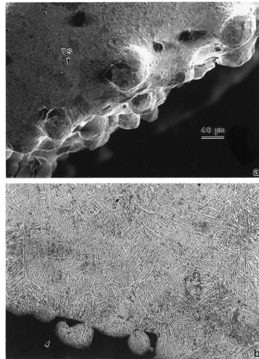
Fig. 10 – Corresponding field emission SEM (a) and optical metallographic section view (b) for the cylindrical build sample in Fig. 9. TS in (a) represents the top surface while the arrow in (b) designates the outer particle surface region. Magnification is shown in (a) for both (a) and (b). (From Murr et al. (in press)).
