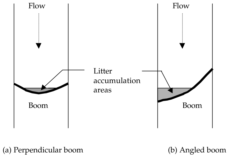
Figure 4.5 - Boom layouts
