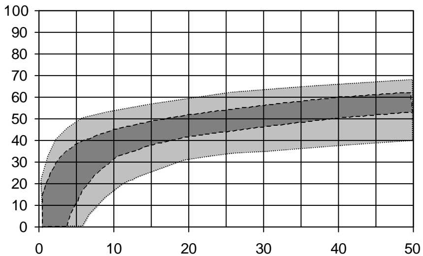
Figure A.2 – Hydraulic residence time relationships
