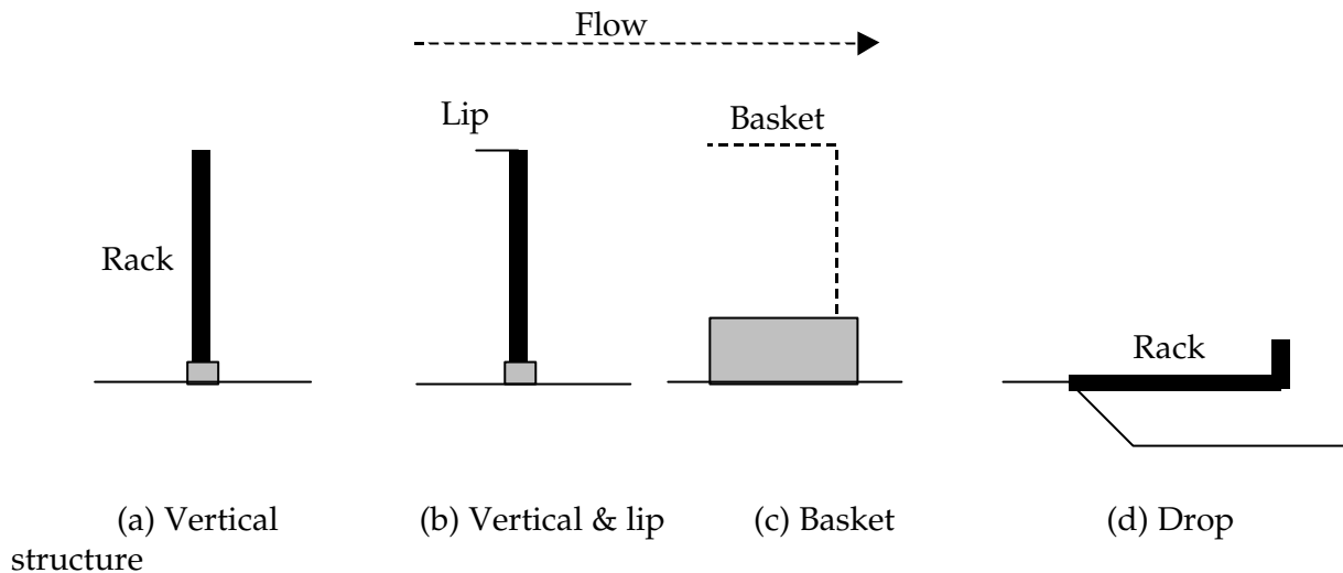
Figure 4.3 – Litter rack sections
