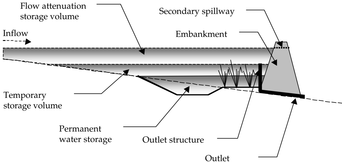
Figure 6.6 – Schematic of an on-line constructed wetland
