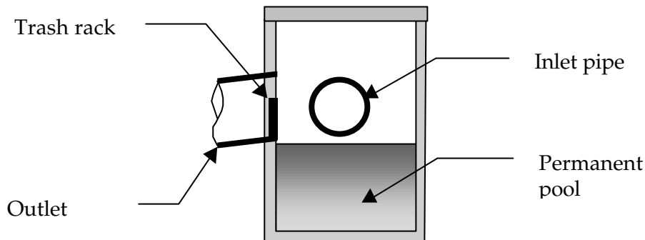
Figure 4.4 – Minor gross pollutant trap
