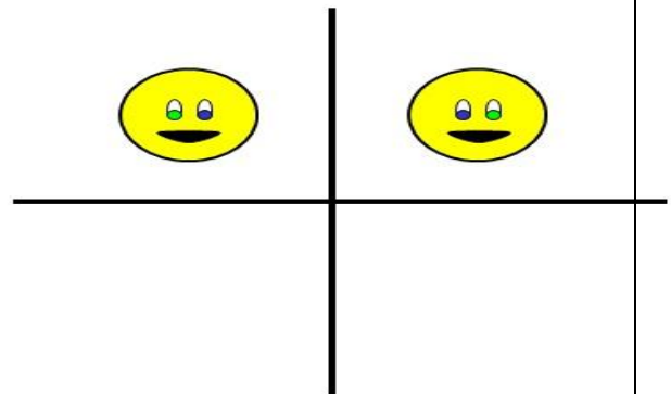
Y-axis reflection
