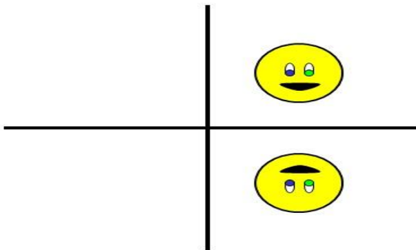
X-axis reflection
