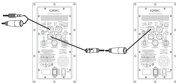
Passing Signal from One KW Series Full-range Model to Another
