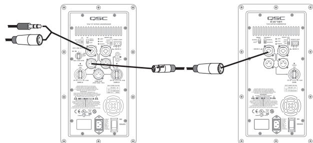
Passing Signal to KW 181
