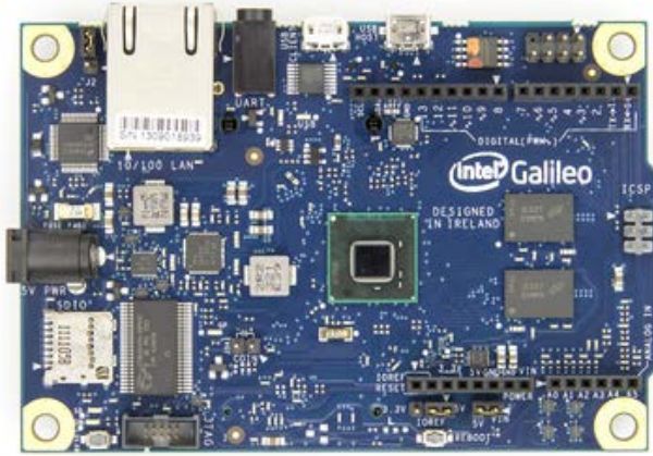
Intel Galileo Front
