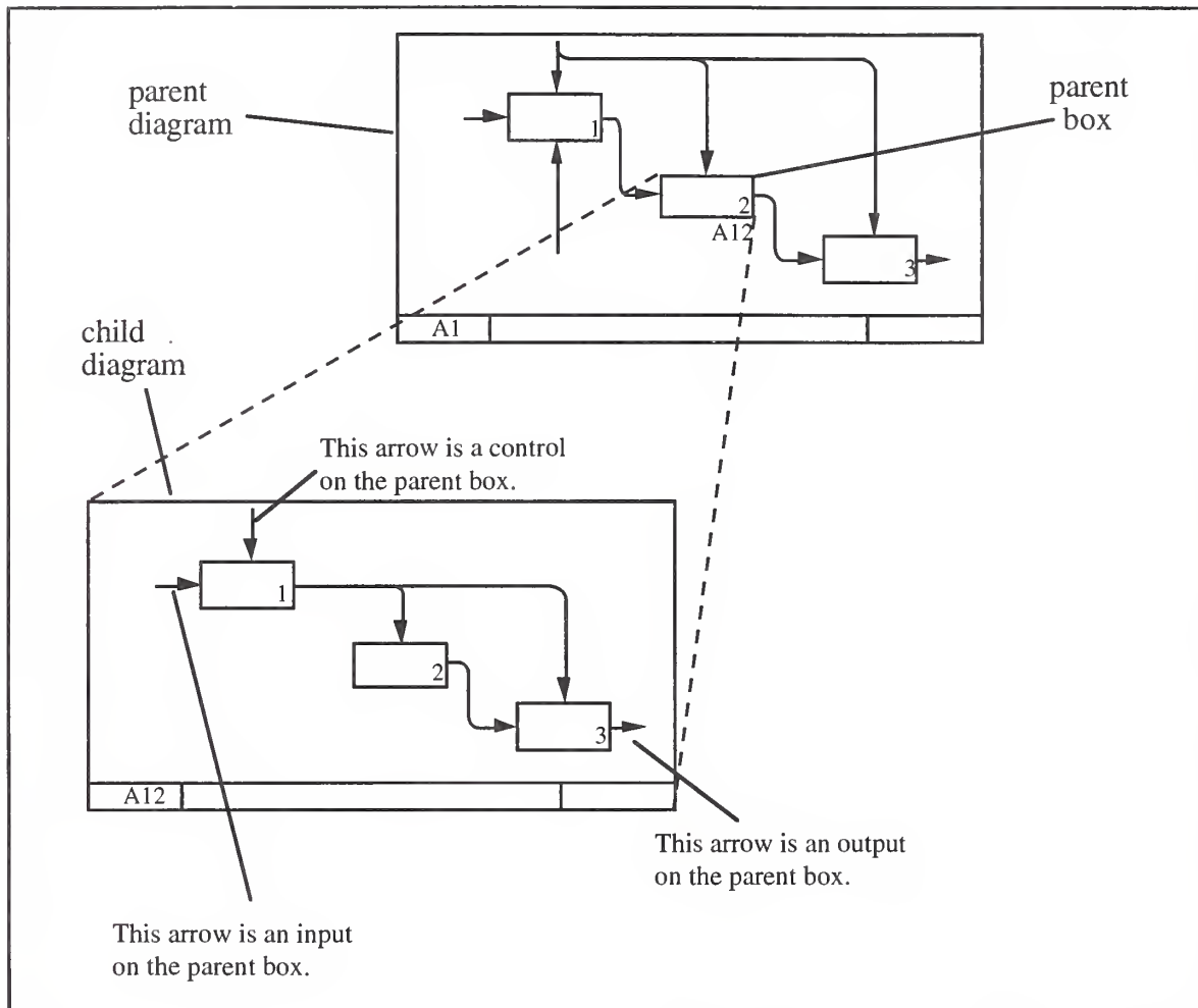
Figure 14. Boundary Arrow Correspondence
