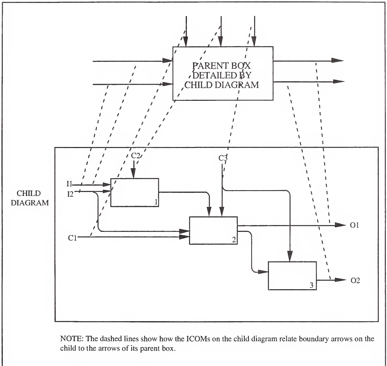
Figure 15. ICOM Codes and Changing Arrow Roles
