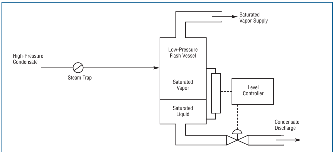
Figure 14. Flash Steam Recovery Vessel
