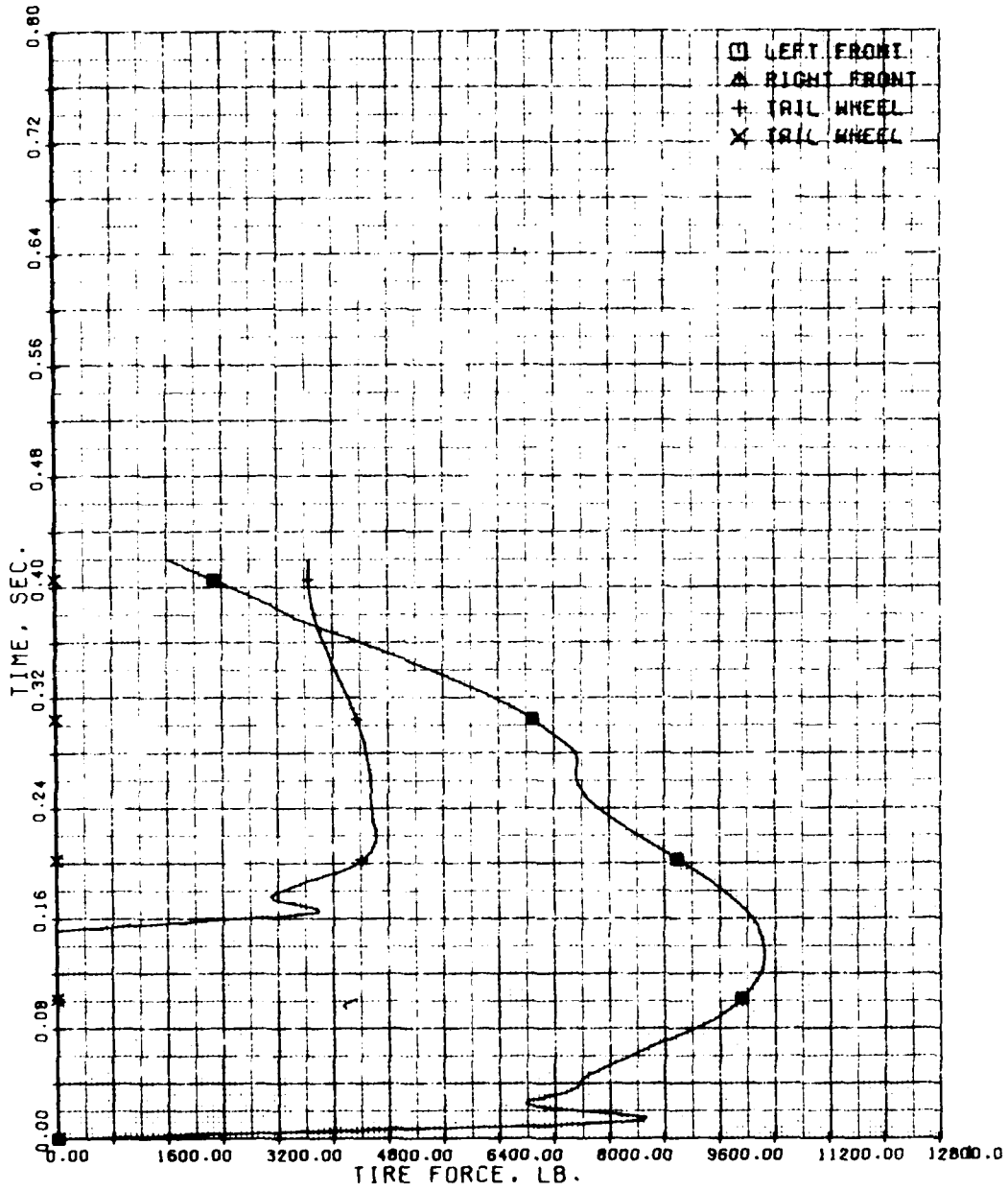
Figure 16. Baseline - 20 ft/sec, -10° pitch, 0° roll.
