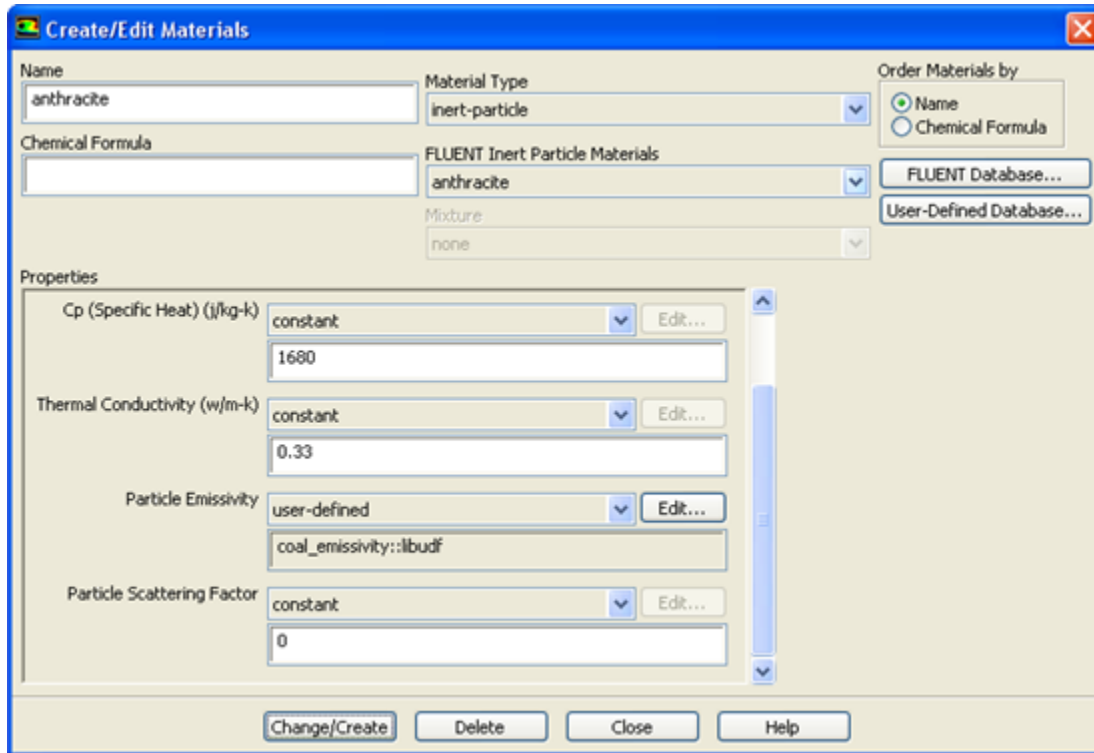
Figure 6.85: The Create/Edit Materials Dialog Box
