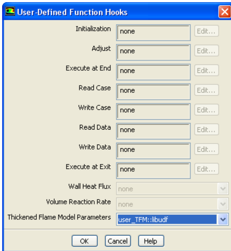
Figure 6.57: The User-Defined Function Hooks Dialog Box
