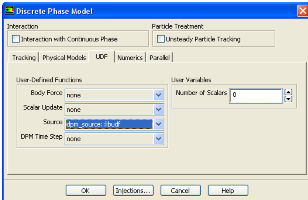
Figure 6.88: The Discrete Phase Model Dialog Box
