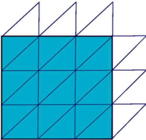
Figure 7.9: Simple Neighborhood Includes the Unfilled Triangles (Connected to the Partition Interface Faces)
