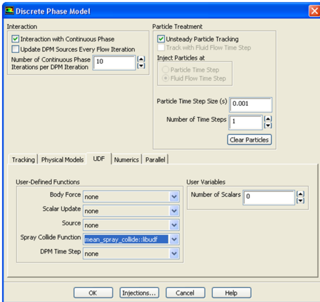
Figure 6.89: The Discrete Phase Model Dialog Box
