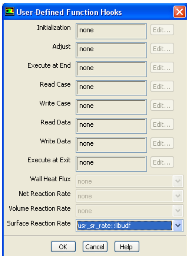
Figure 6.56: The User-Defined Function Hooks Dialog Box
