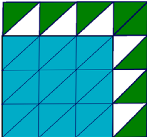
Figure 7.10: Extended Neighborhood Includes the Unfilled Triangles and the Green Triangles (Connected to the Partition Interface Nodes)
