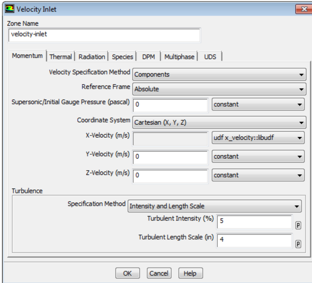
Figure 6.36: The Velocity Inlet Dialog Box
