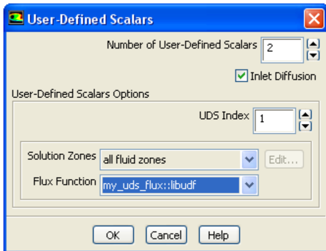
Figure 6.103: The User-Defined Scalars Dialog Box
