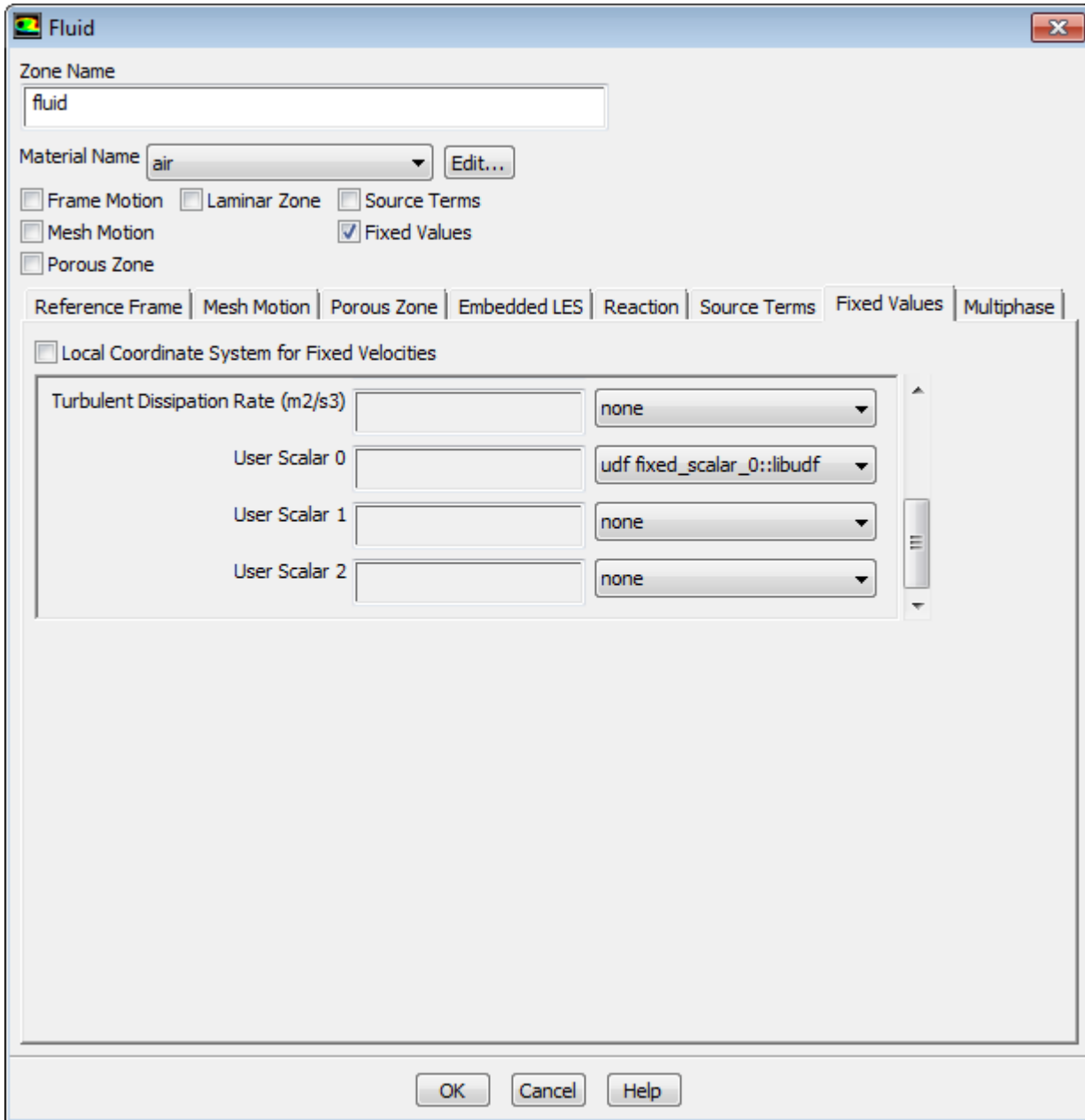
Figure 6.37: The Fluid Dialog Box with Fixed Value Inputs for User-Defined Scalars
