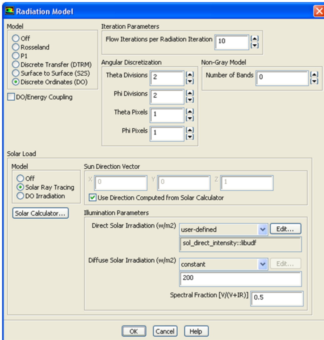
Figure 6.44: The Radiation Model Dialog Box
