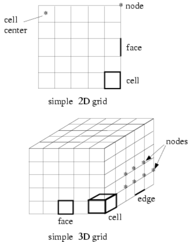
Figure 1.1: Mesh Components
