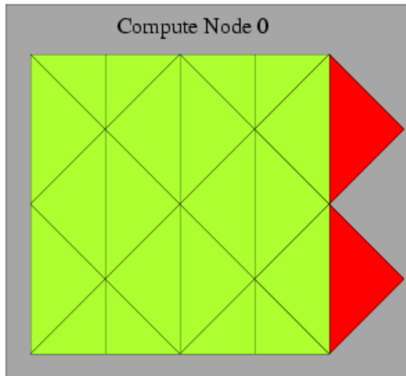
Figure 7.11: Looping Over Interior Cells in a Partitioned Mesh Using begin,end_c_loop_int (indicated by the green cells)
