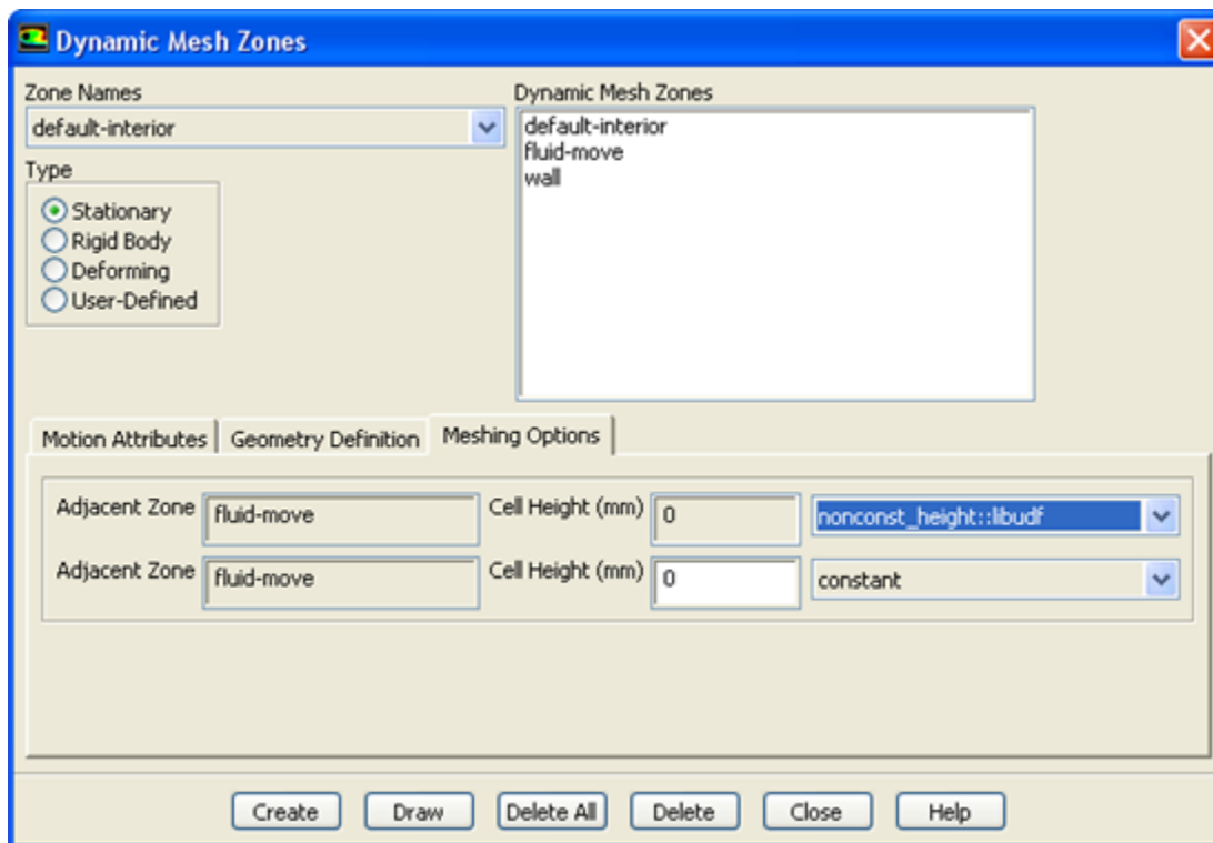
Figure 6.96: The Dynamic Mesh Zones Dialog Box
