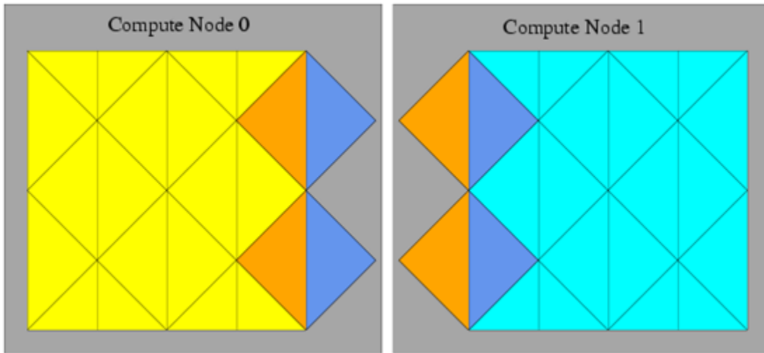
Figure 7.2: Partitioned Mesh Distributed Between Two Compute Nodes
