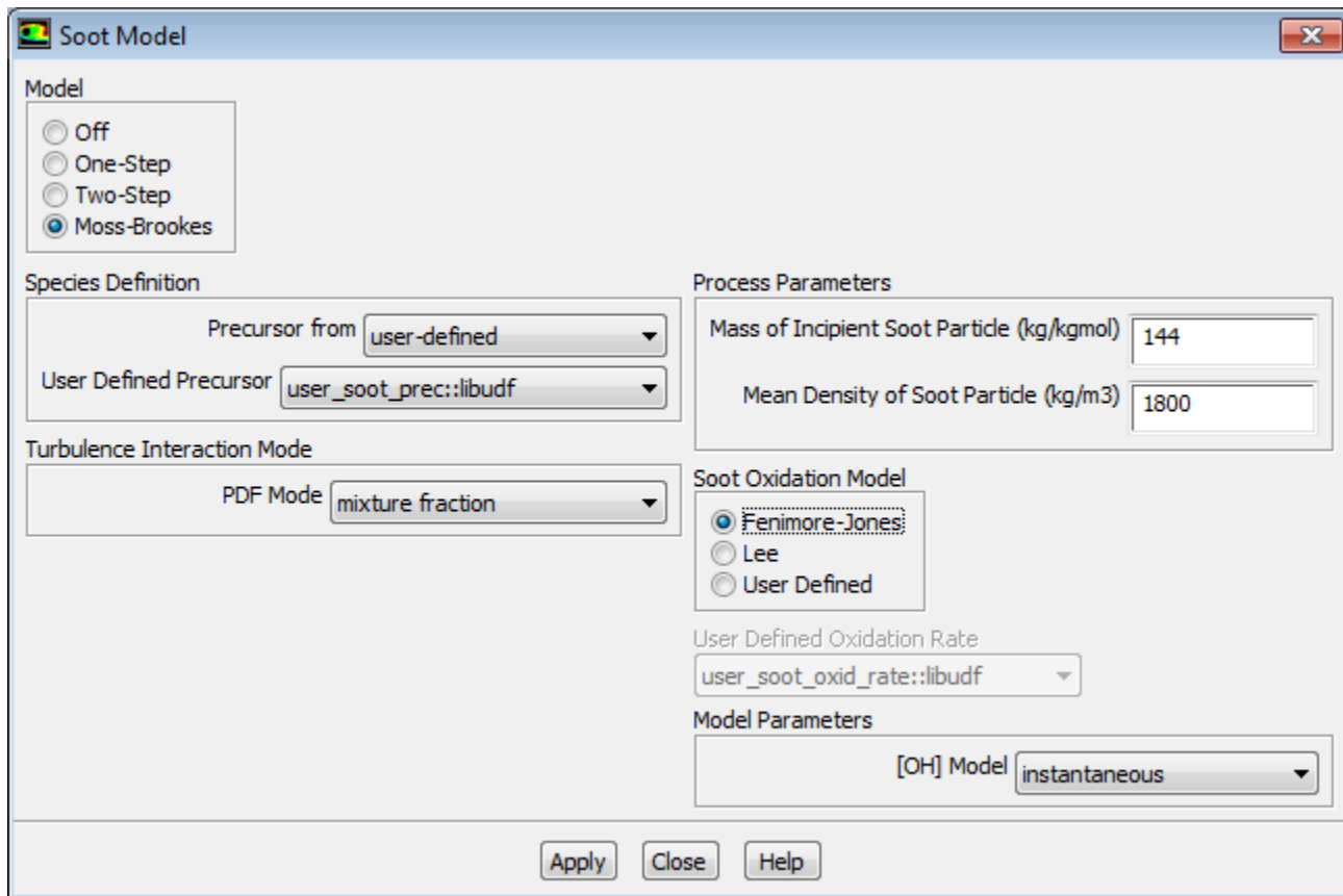
Figure 6.51: The Soot Model Dialog Box (User-Defined Precursor)
