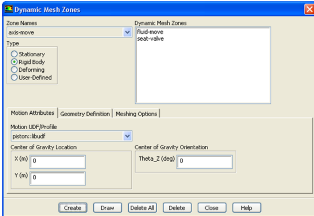
Figure 6.94: The Dynamic Mesh Zones Dialog Box
