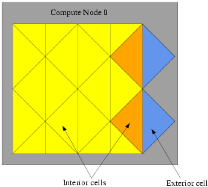
Figure 7.6: Partitioned Mesh: Cells
