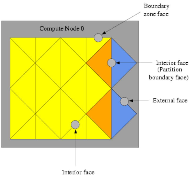
Figure 7.7: Partitioned Mesh: Faces
