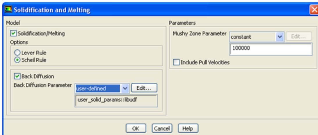
Figure 6.46: The Solidification and Melting Dialog Box
