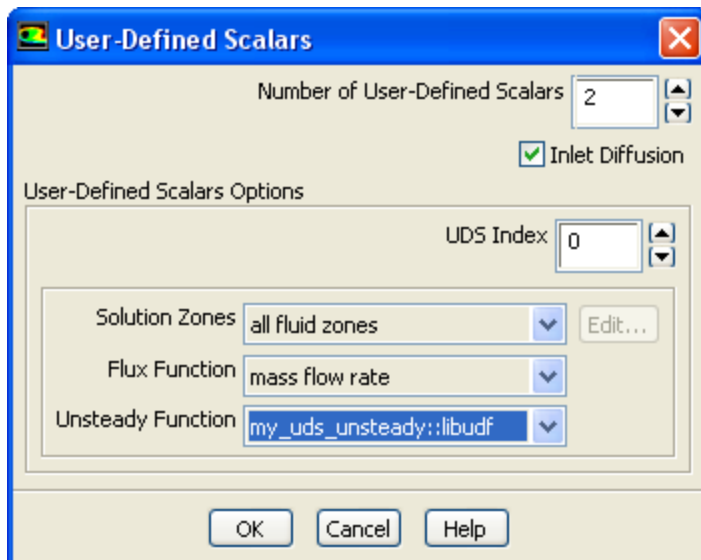
Figure 6.104: The User-Defined Scalars Dialog Box
