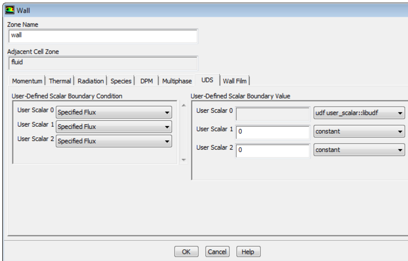
Figure 6.38: The Wall Dialog Box with Inputs for User-Defined Scalars
