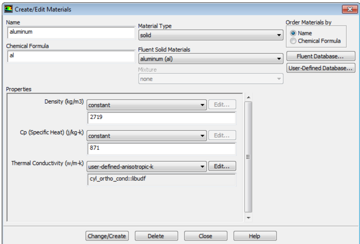
Figure 6.14: The Create/Edit Materials Dialog Box
