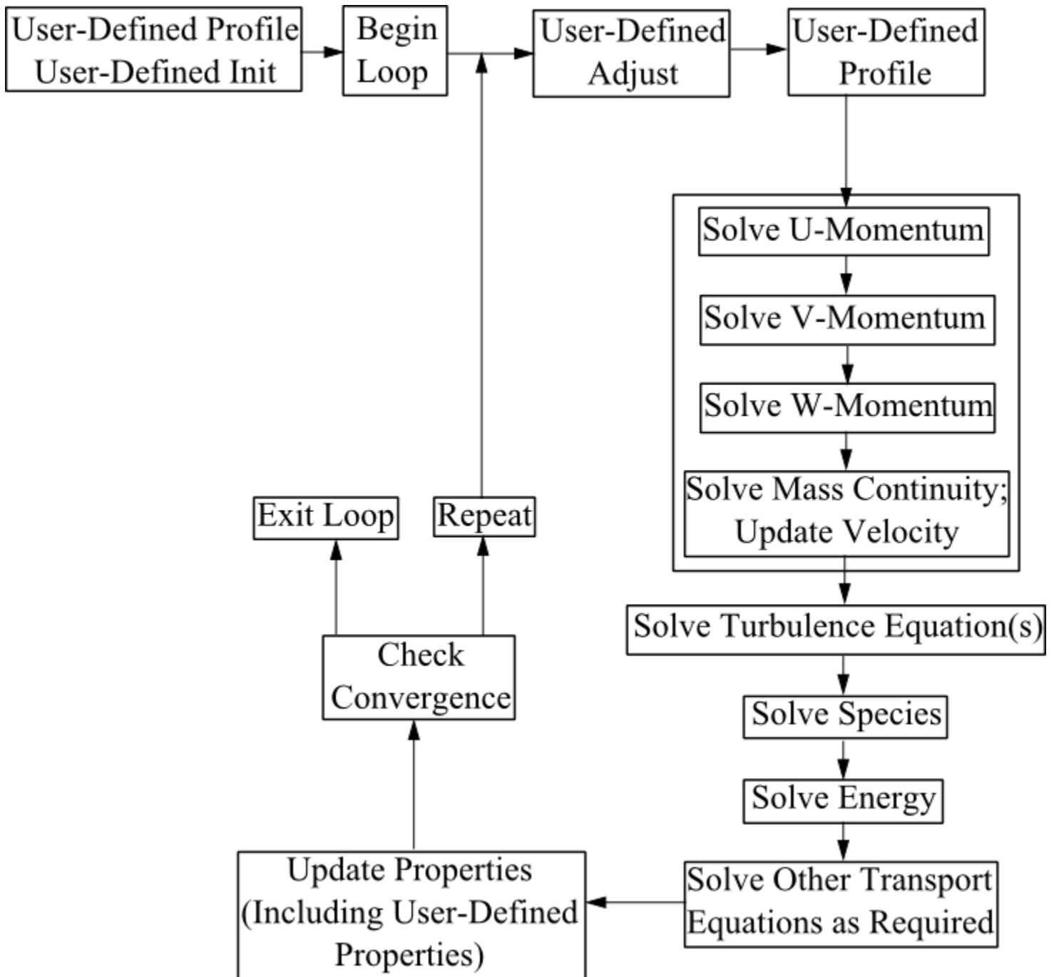
Figure 1.2: Solution Procedure for the Pressure-Based Segregated Solver
