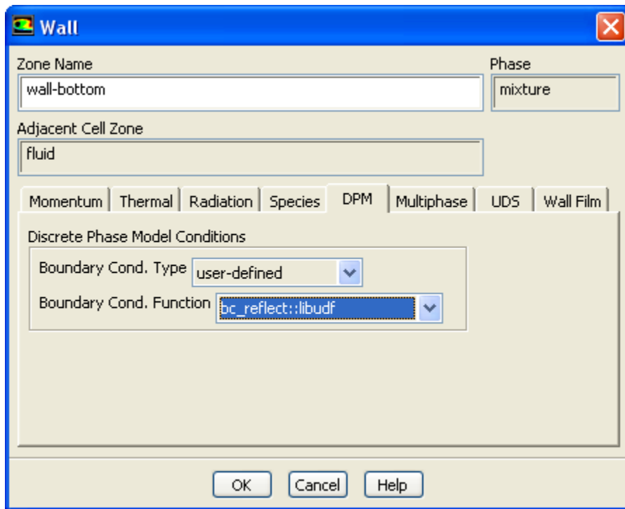
Figure 6.77: The Wall Dialog Box
