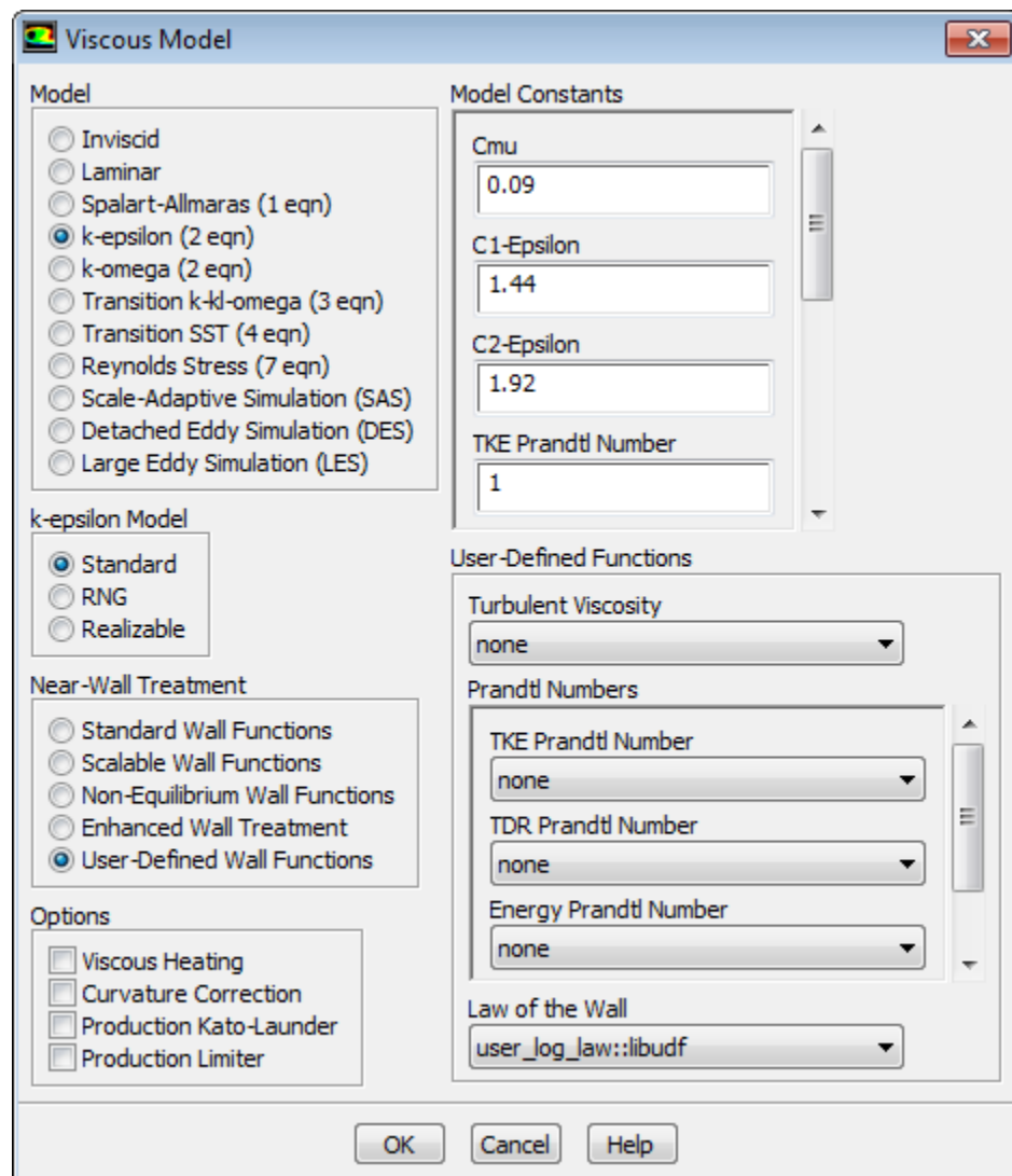
Figure 6.64: The Viscous Model Dialog Box
