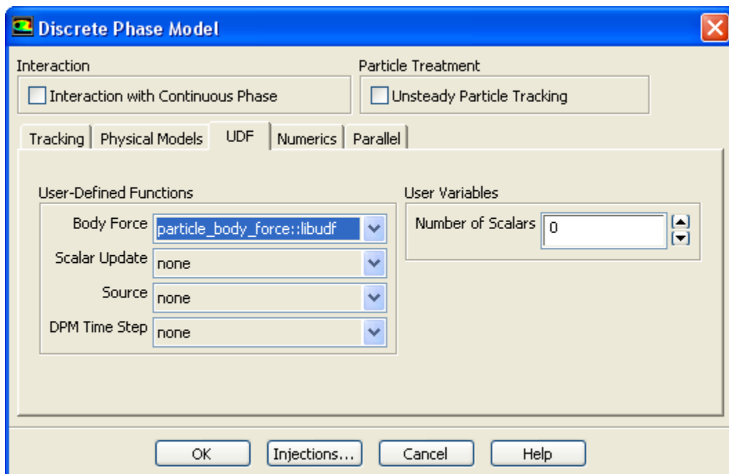
Figure 6.78: The Discrete Phase Model Dialog Box
