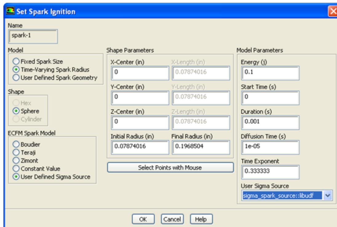
Figure 6.24: The Set Spark Ignition Dialog Box
