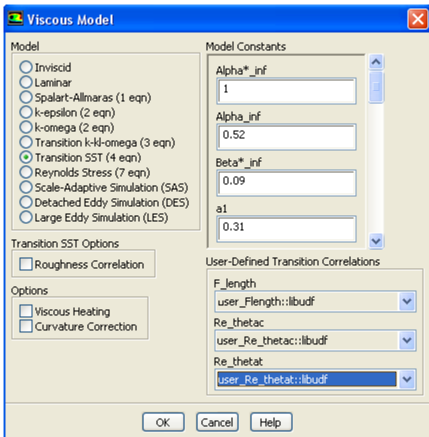
Figure 6.58: The Viscous Model Dialog Box
