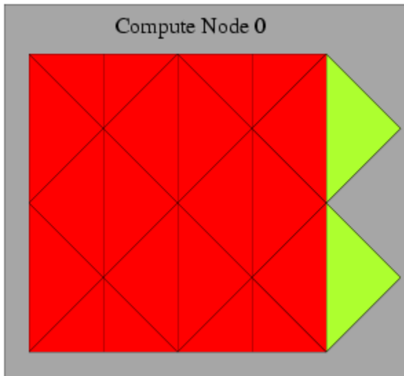
Figure 7.12: Looping Over Exterior Cells in a Partitioned Mesh Using begin,end_c_loop_ext (indicated by the green cells)
