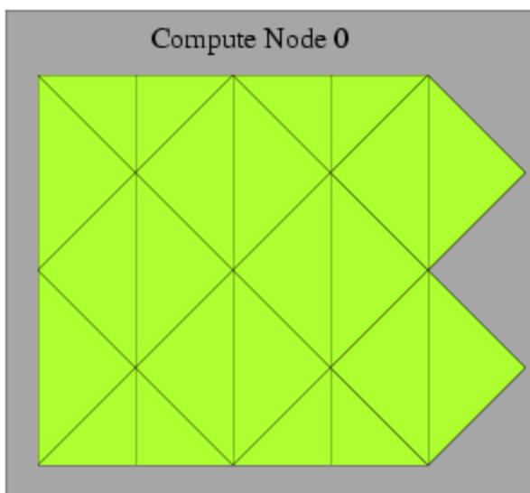
Figure 7.13: Looping Over Both Interior and Exterior Cells in a Partitioned Mesh Using begin,end_c_loop
