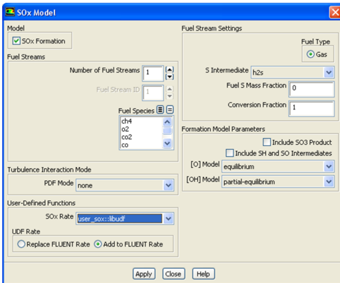
Figure 6.52: The SOx Model Dialog Box
