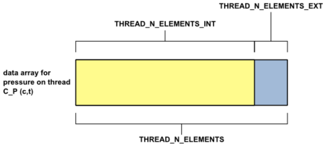
Figure 7.8: Exterior Thread Data Storage at End of a Thread Array
