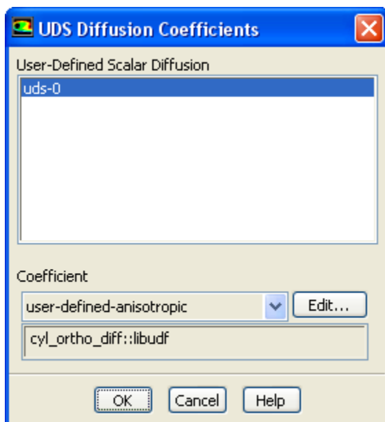
Figure 6.102: The UDS Diffusion Coefficients Dialog Box
