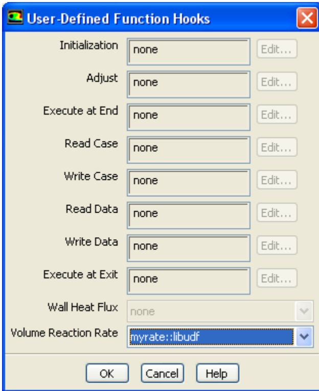
Figure 6.63: The User-Defined Function Hooks Dialog Box
