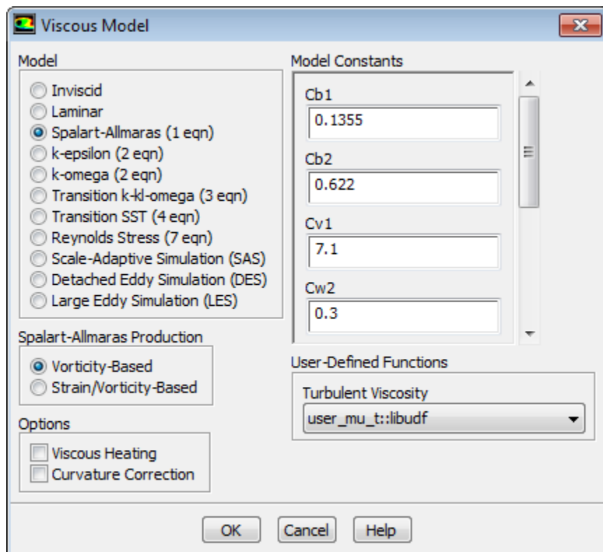
Figure 6.62: The Viscous Model Dialog Box
