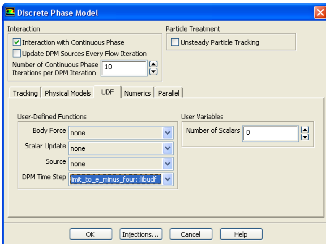
Figure 6.91: The Discrete Phase Model Dialog Box
