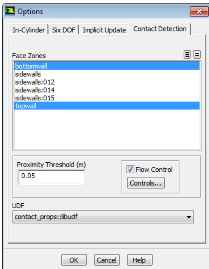
Figure 6.100: The Options Dialog Box Showing the Contact Detection Tab
