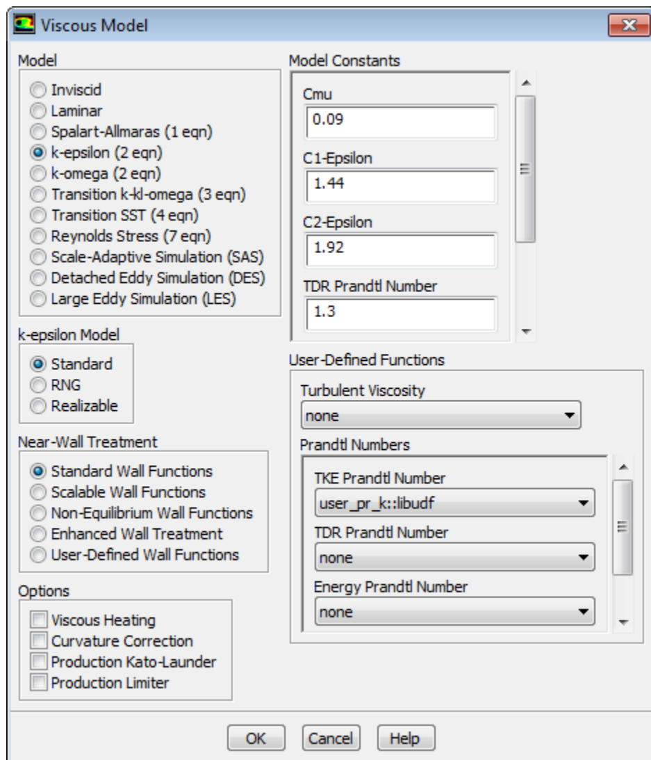
Figure 6.35: The Viscous Model Dialog Box
