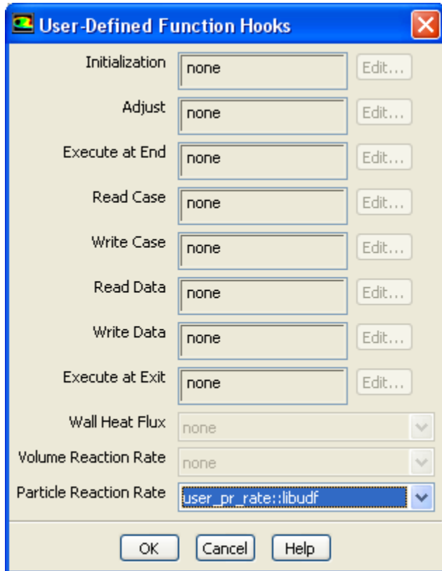
Figure 6.34: The User-Defined Function Hooks Dialog Box
