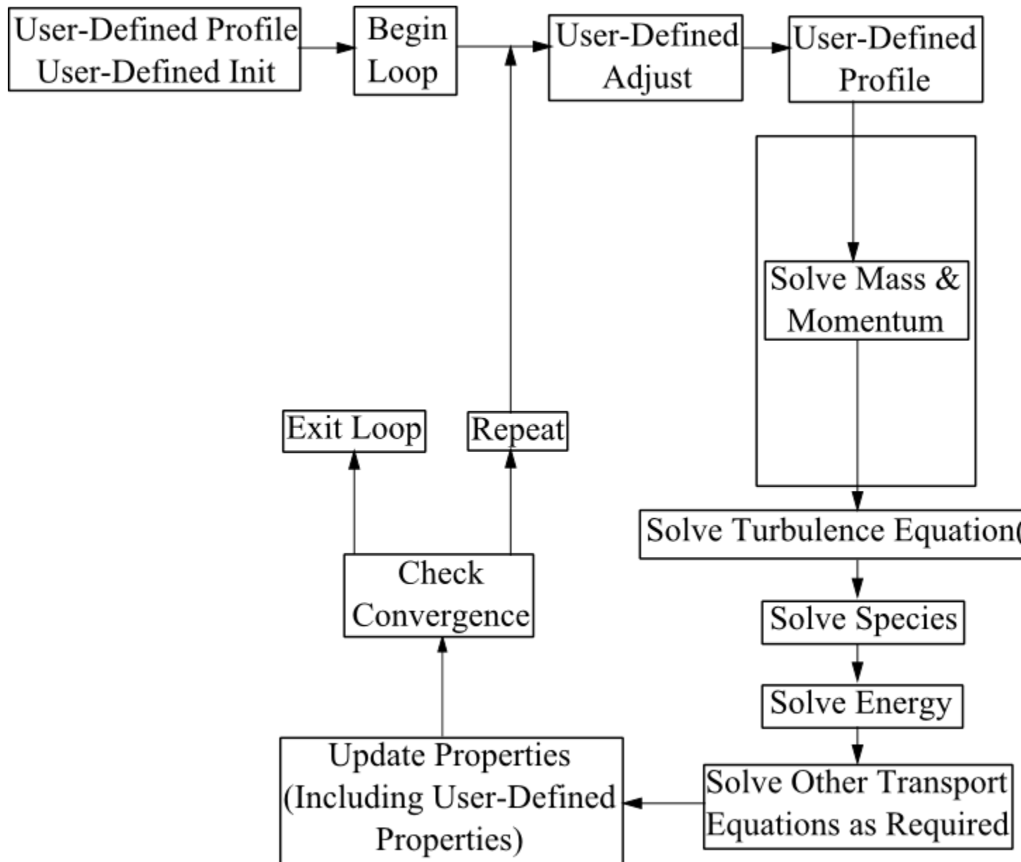
Figure 1.3: Solution Procedure for the Pressure-Based Coupled Solver
