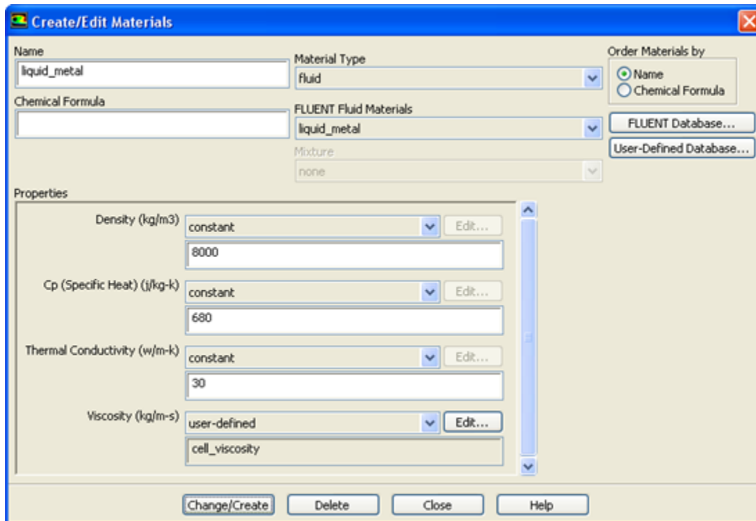
Figure 6.39: The Create/ Edit Materials Dialog Box
