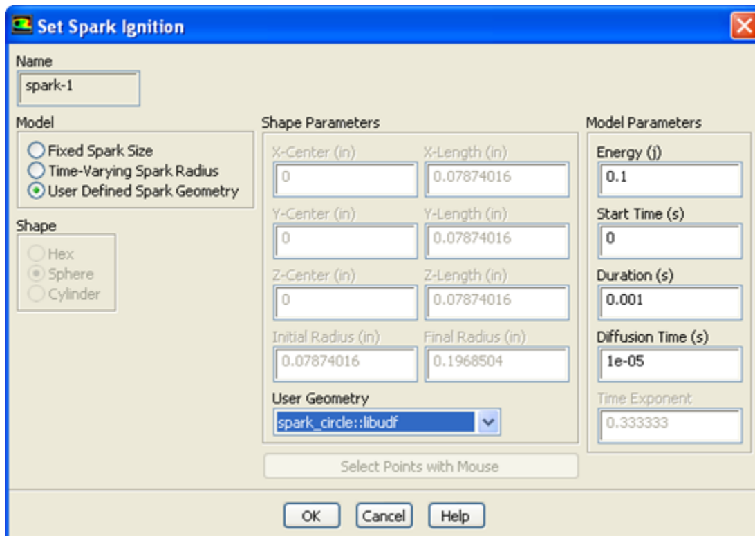
Figure 6.53: The Set Spark Ignition Dialog Box
