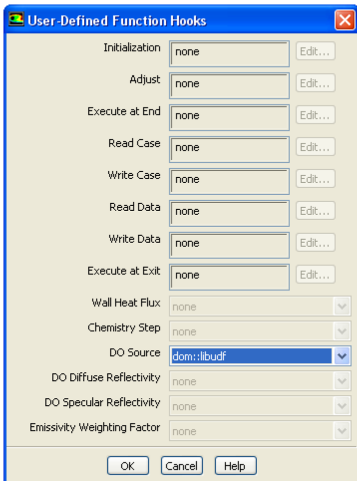
Figure 6.22: The User-Defined Function Hooks Dialog Box
