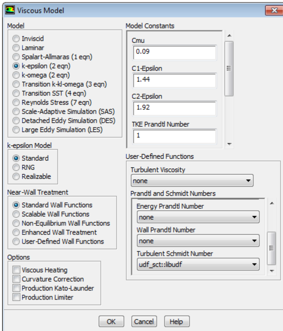
Figure 6.61: The Viscous Model Dialog Box
