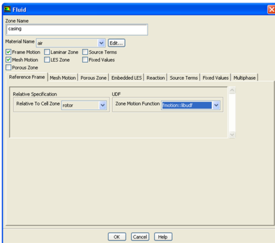
Figure 6.26: The Fluid Dialog Box for Frame Motion
