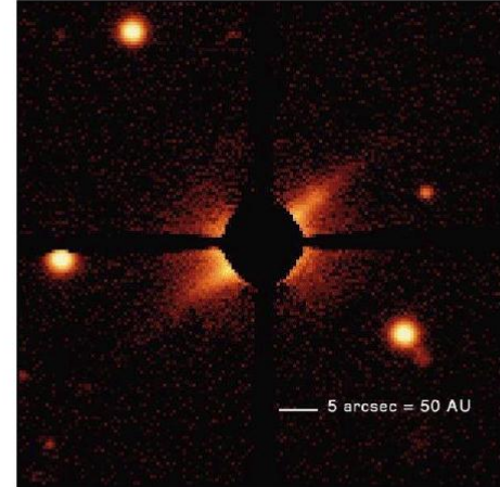
Fig. 1.— The disk surrounding AU Mic seen in optical scattered light. North is up, east is left, and each side of this false-color image corresponds to 60'' . The central dark region is produced by the 9.5'' diameter focal plane occulting spot which is suspended by four wires and completely masks our direct view of the star. This image represents 900 seconds total integration in the R band and each pixel corresponds to 4 AU at the distance to AU Mic. Residual light evident near the occulting spot edge in the NE-SW direction is attributed to asymmetries in the point-spread function caused by instrumental scattering and atmospheric seeing.
