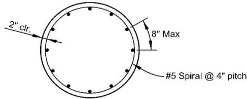
Figure 4 - Column Confinement Reinforcement
