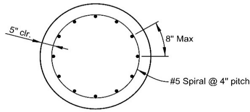
Figure 5 - Caisson Confinement Reinforcement
