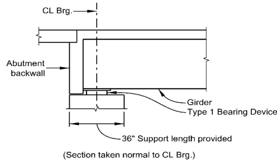
Figure 3 - Abutment Support Length
