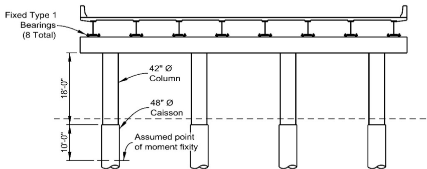
Figure 2 - Pier 2 Elevation
