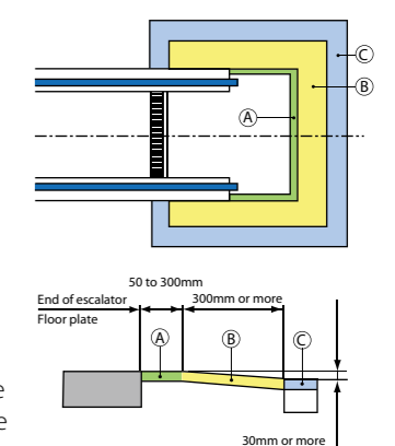
Detailed floor plan for outdoor escalators
