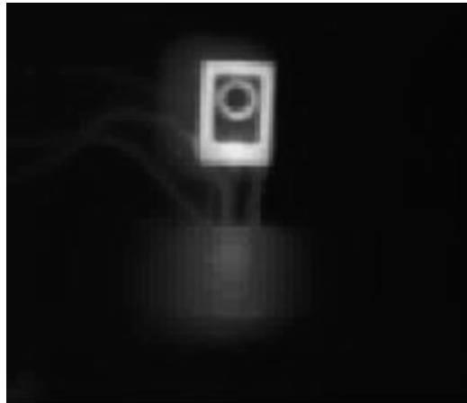
Figure 2. Through-hole transistor in TO-32 case with maximum case temperatures of 163°C.
