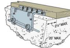
UFP10 installed on a Trapezoid Foundation
