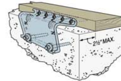
UFP10 installed on a Straight Foundation
