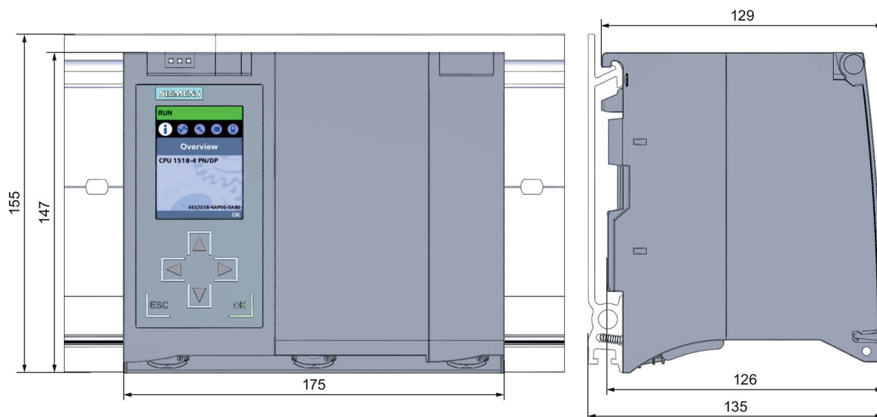
Figure A-1 Dimensional drawing of CPU 1518-4 PN/DP, front and side views
