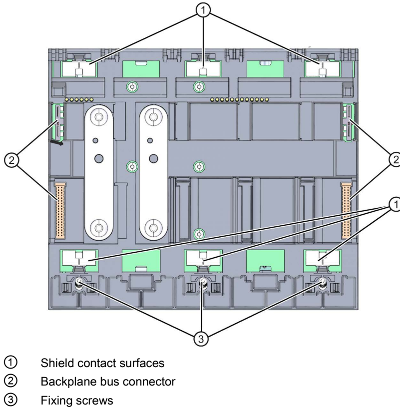
Figure 2-5 View of the CPU 1518-4 PN/DP - rear
