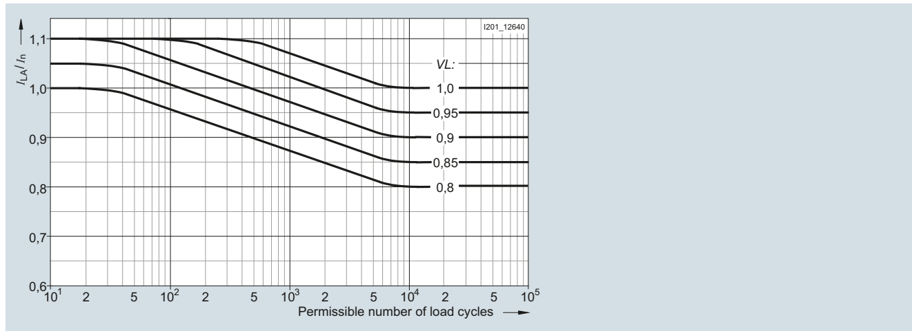
Waveform of the varying load factor V_L for load cycles
