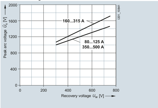
Peak arc voltage
