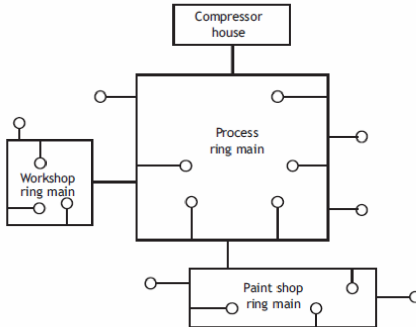
Ring Main with Take-off Points
