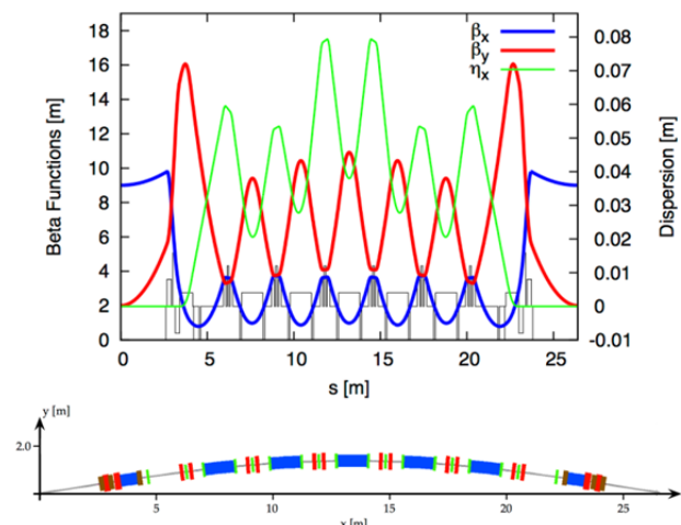
Figure 3: MAX IV 3 GeV achromat and optics.
