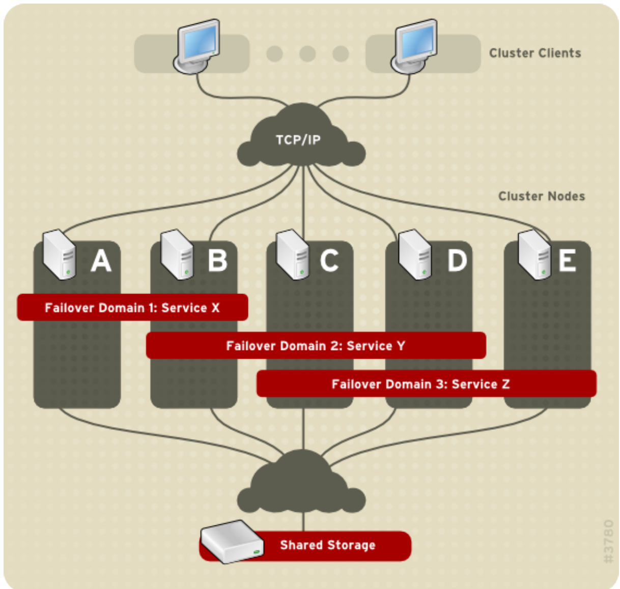
Figure 1.9. Failover Domains
