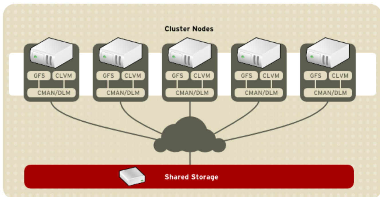
Figure 1.2. CMAN/DLM Overview
