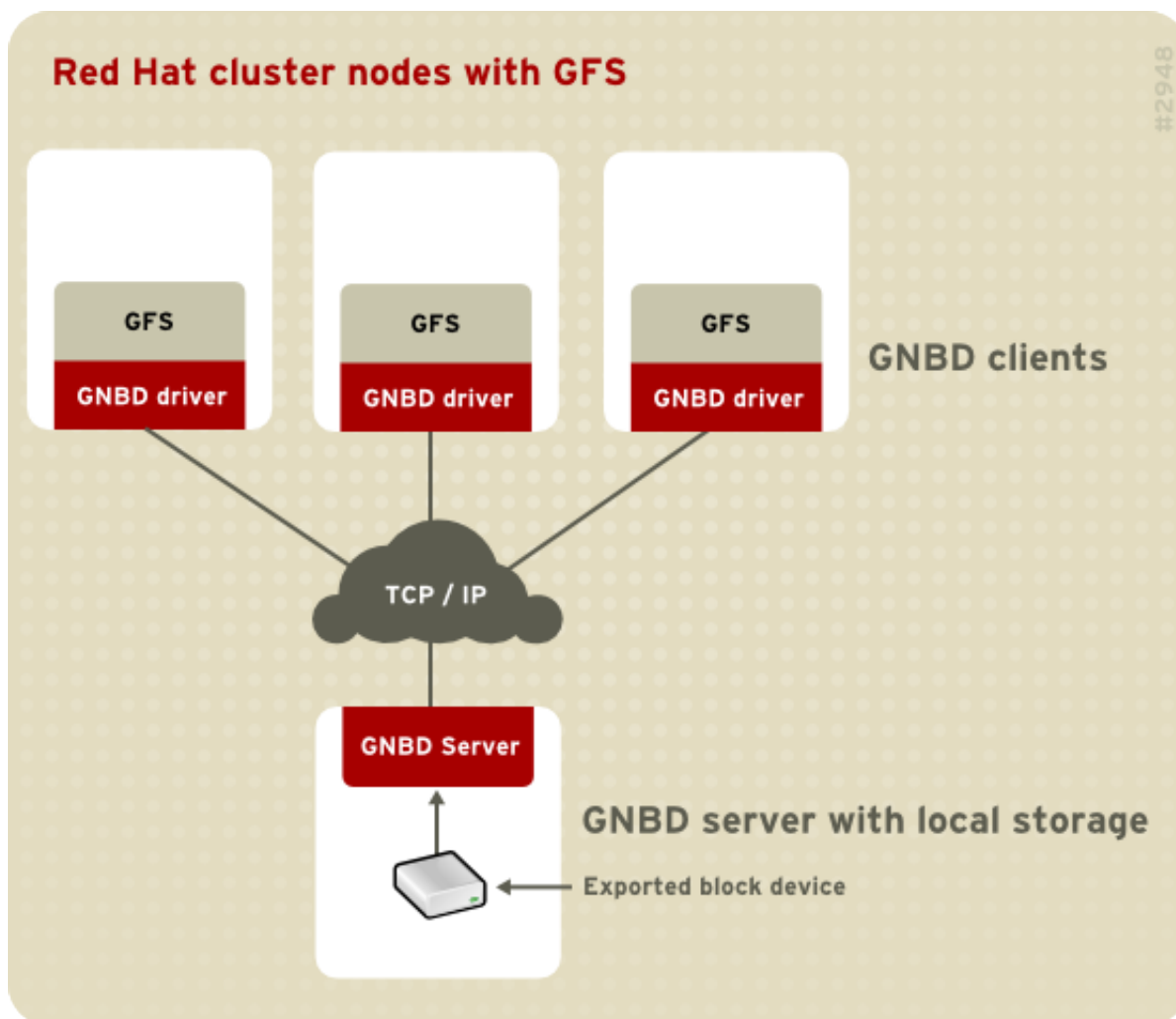
Figure 1.15. GNBD Overview
