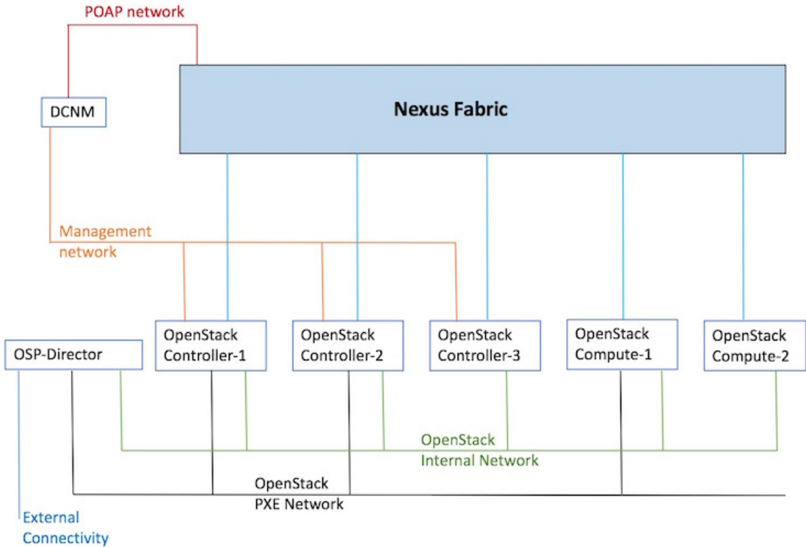
Figure 3: Sample topology
