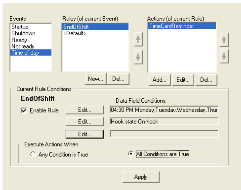
Figure 40. Work Flow window
