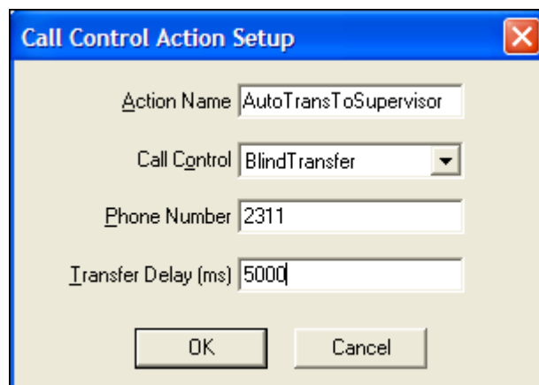
Figure 52. Call Control Action Setup dialog box
