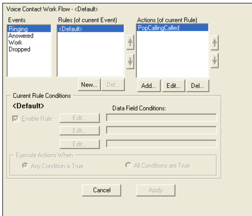
Figure 36. Voice Contact Work Flow window
