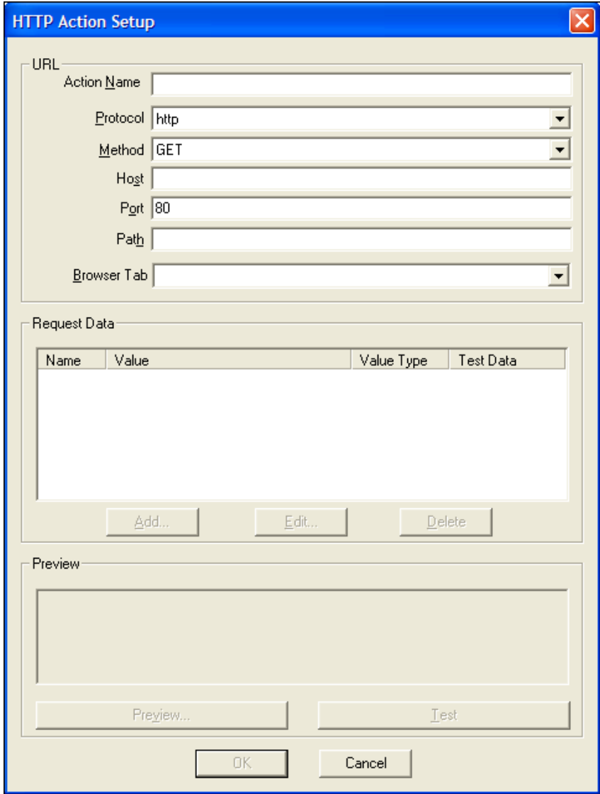
Figure 54. HTTP Actions Setup dialog box
