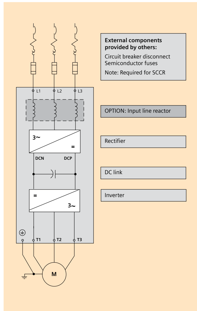
Typical power circuit of SINAMICS G150 type C enclosed chassis
