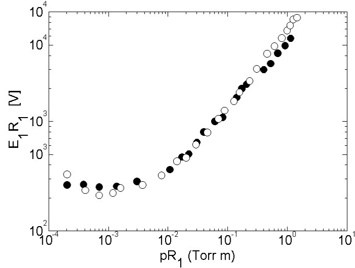
Figure 9. Similarity theorem for corona onset in dry air
