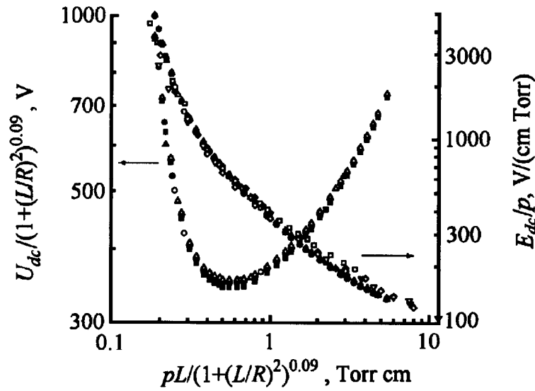
Figure 5. Dependence of breakdown voltage U_{dc} and breakdown field E_{dc}/p on pL in air with discharge tube radius 3.15 cm and different gaps (from 0.5 to 10 cm (theoretical), and comparison with measured data
