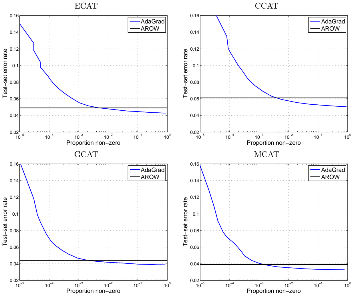
Figure 7: Test set error rates as a function of proportion of non-zeros in predictor x output by ADAGRAD (AROW plotted for reference).
