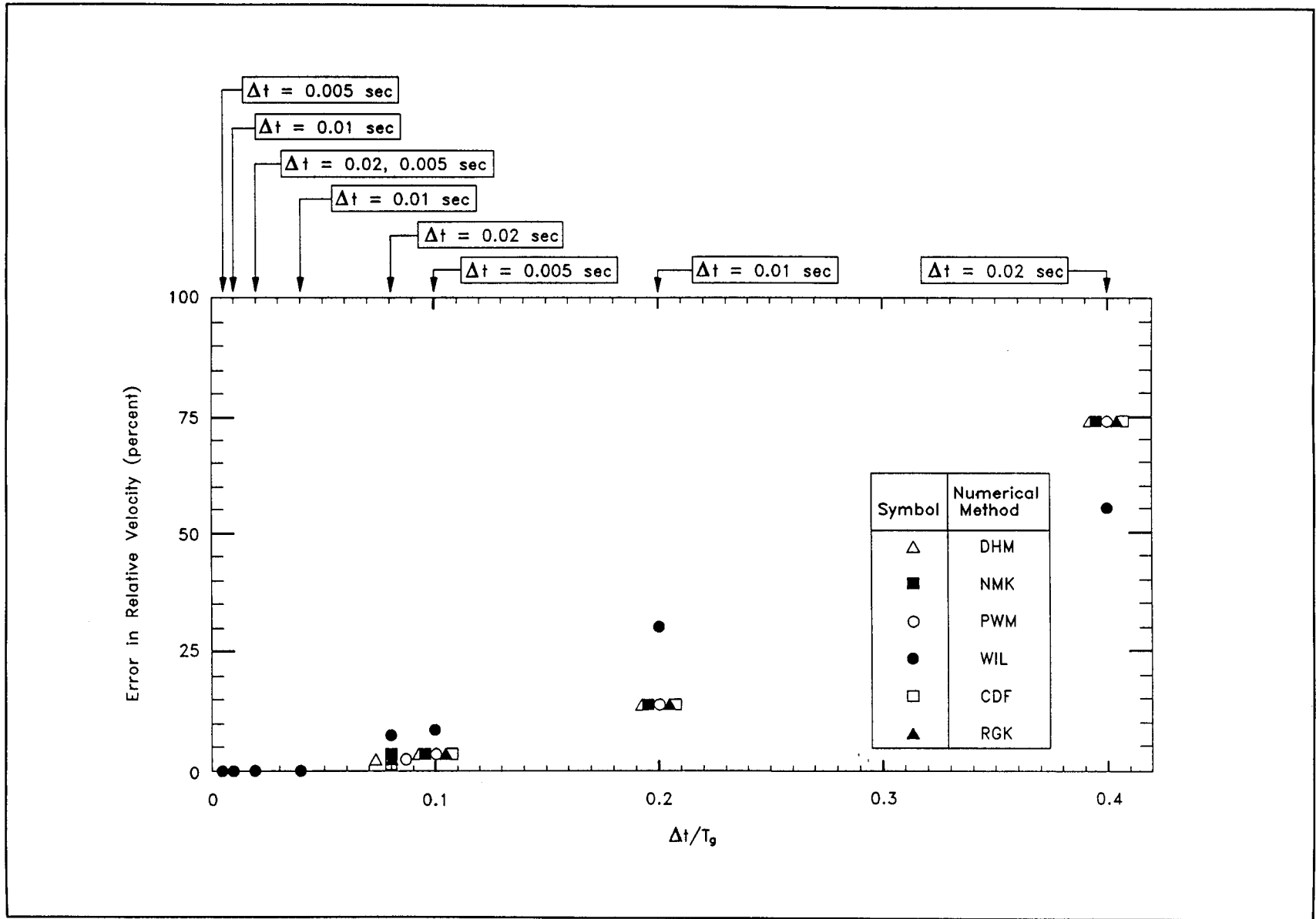
Figure 18. Percentile errors in maximum relative velocity (peak or valley value) for SDOF system of T_0 = 0.5 sec
