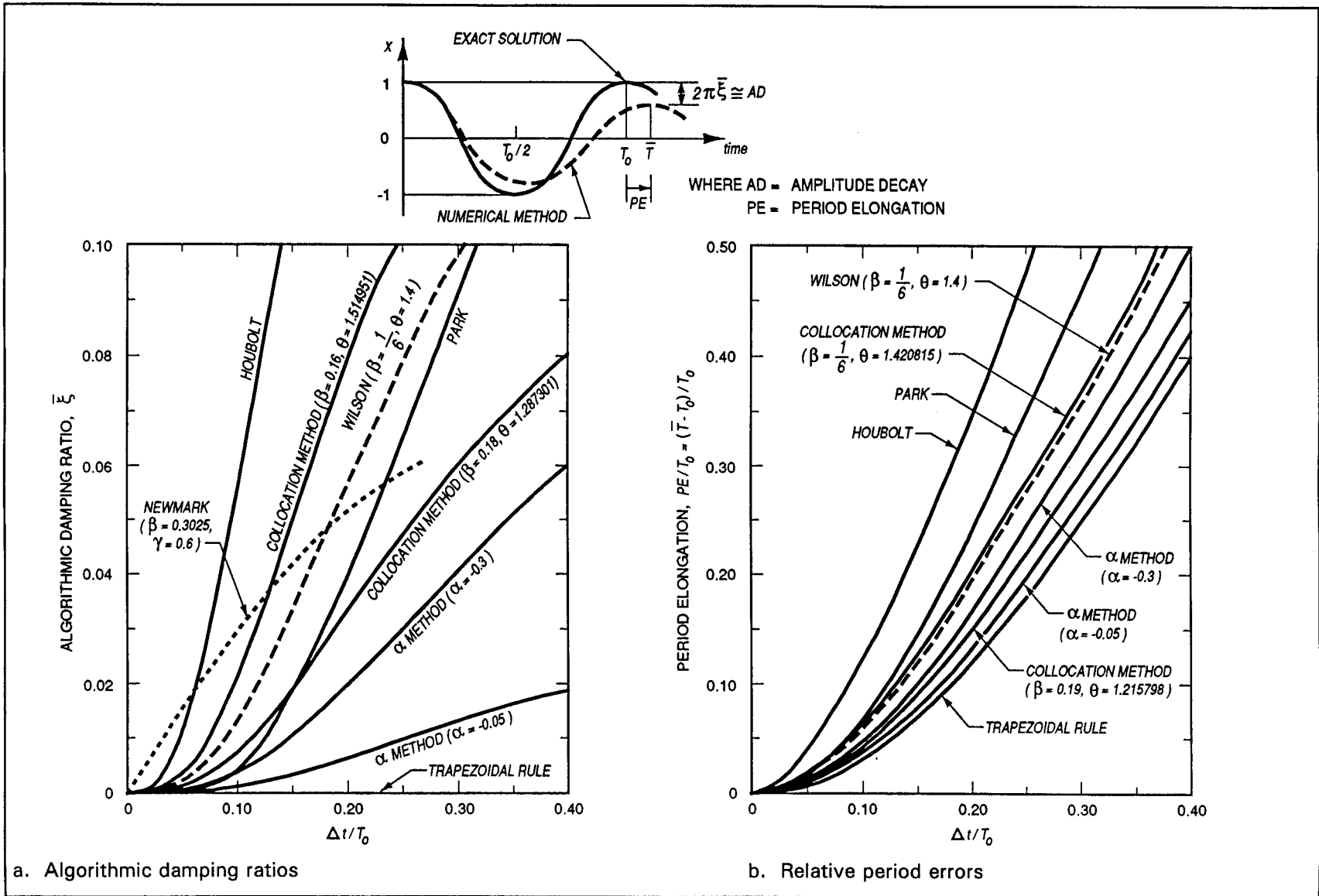
Figure 6. Errors in free vibration response of SDOF systems for \alpha -methods, optimal collocation schemes, and Houbolt, Newmark, Park, and Wilson methods (Courtesy of Hughes 1987)
