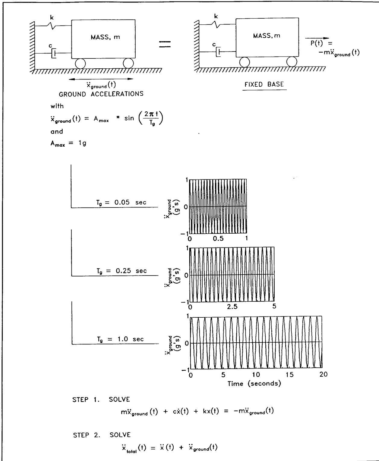
Figure 7. Equivalent dynamic SDOF system problems
