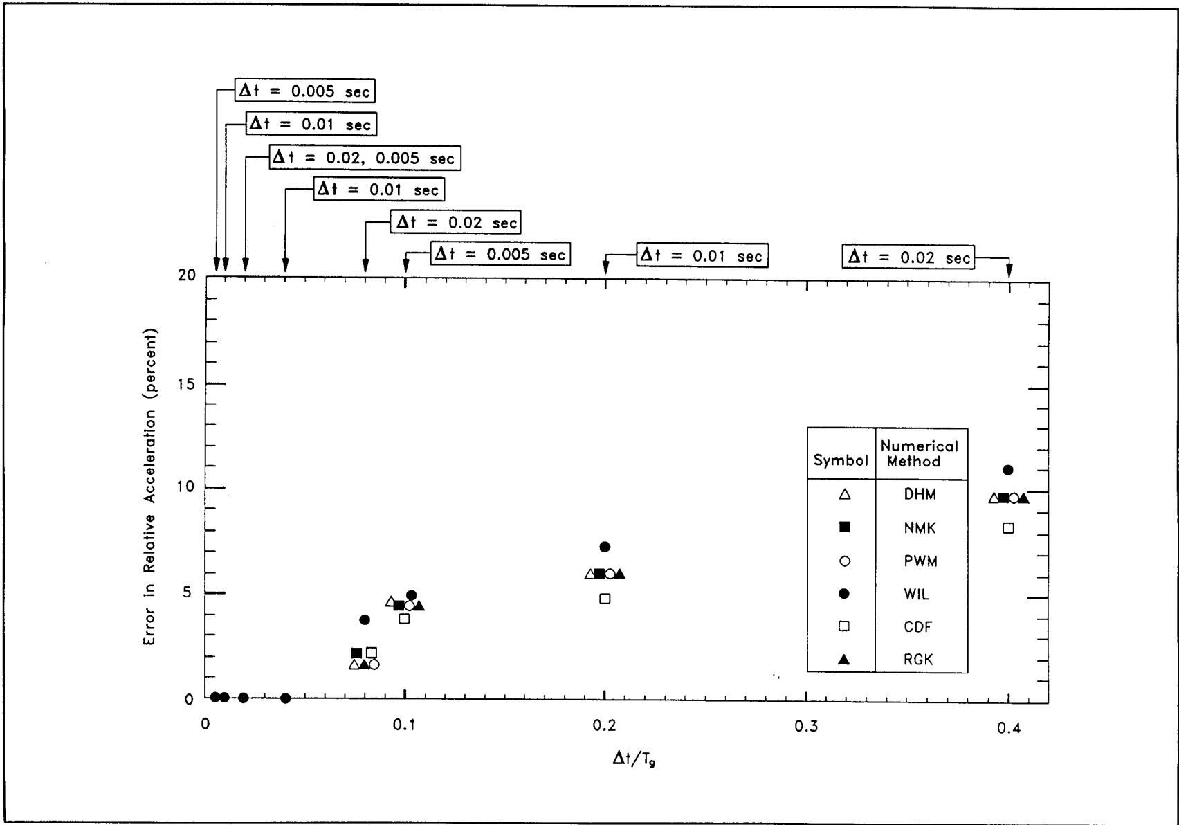
Figure 19. Percentile errors in maximum relative acceleration (peak or valley value) for SDOF system of T_0 = 0.5 sec
