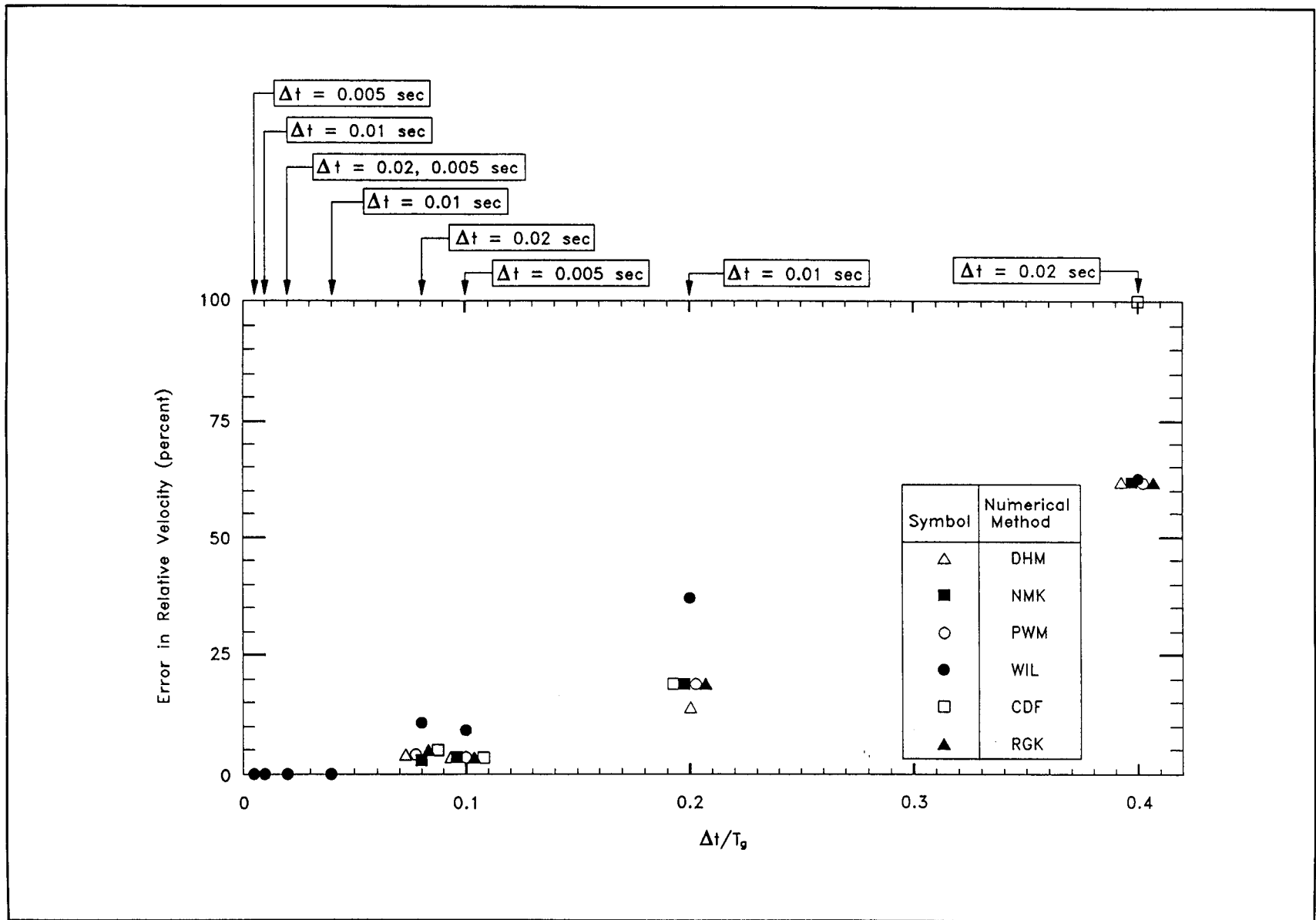
Figure 14. Percentile errors in maximum relative velocity (peak or valley value) for SDOF system of T_0 = 0.25 sec
