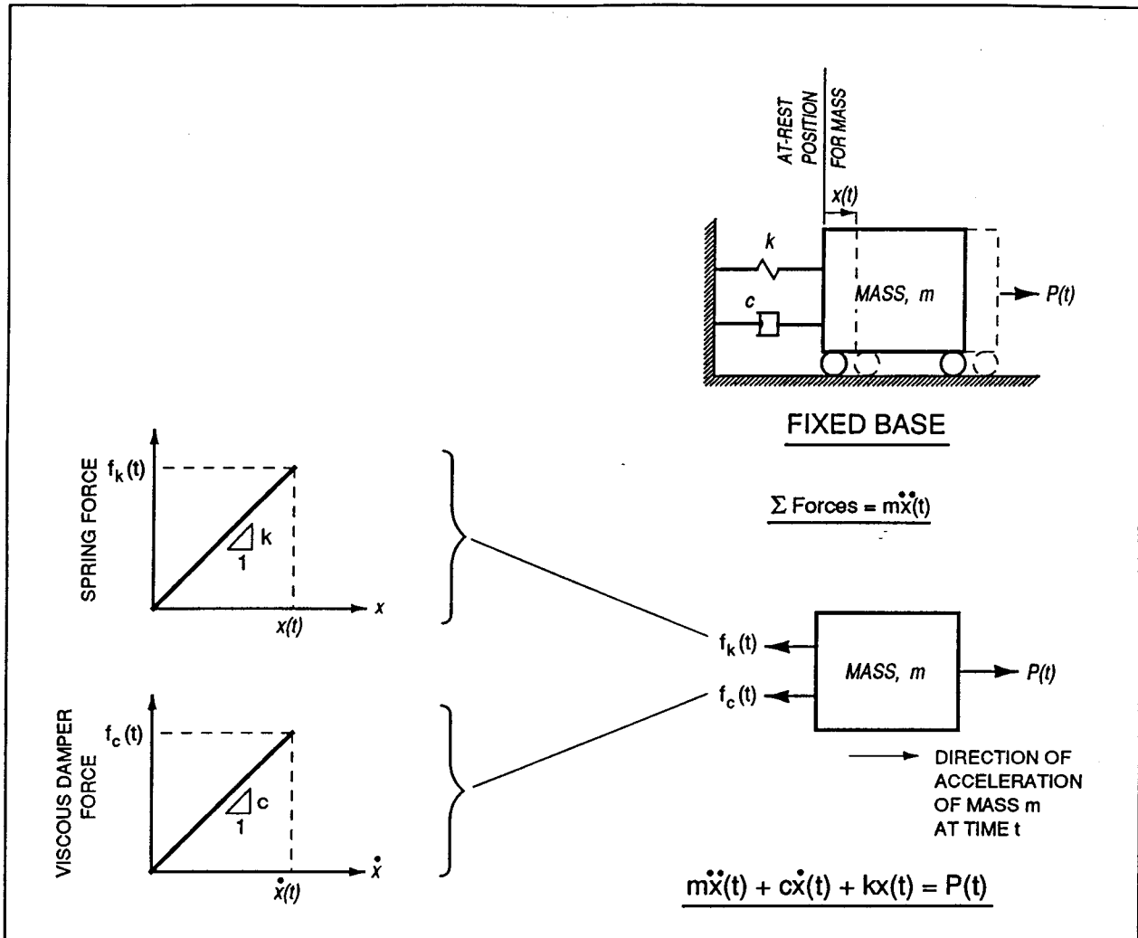
Figure 2. Forces acting on linear SDOF system at time t , external force P(t) applied (Ebeling 1992)
