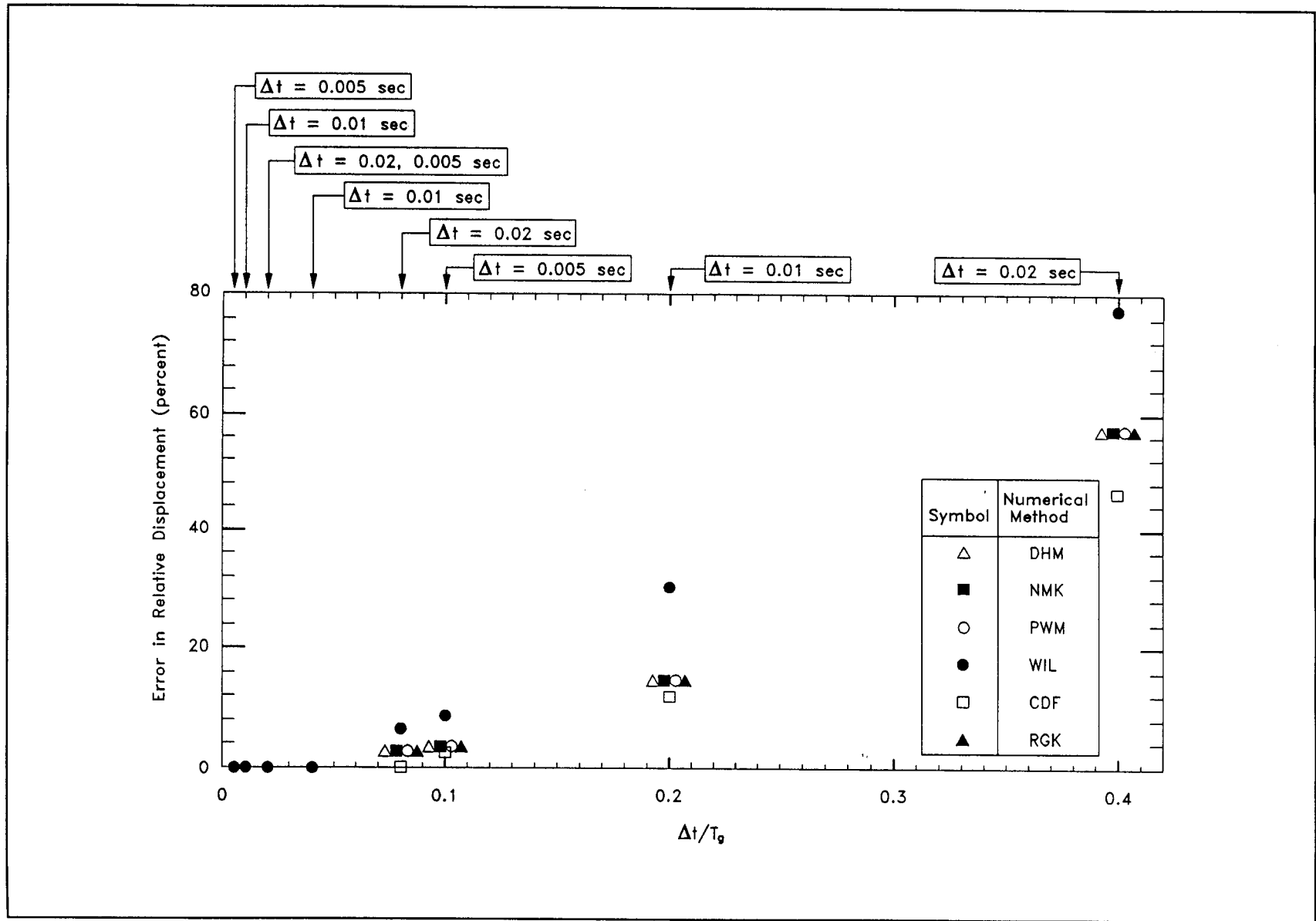
Figure 17. Percentile errors in maximum relative displacements (peak or valley value) for SDOF system of T_0 = 0.5 sec
