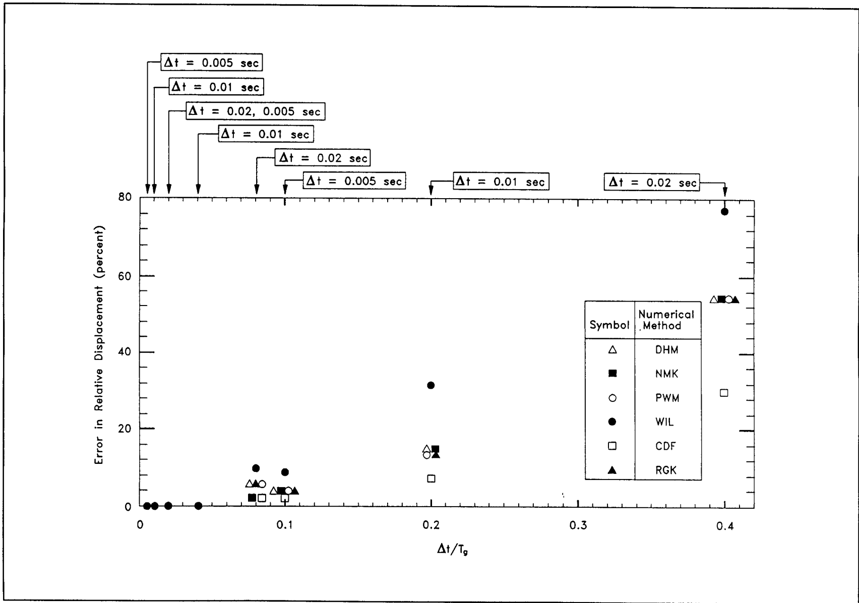
Figure 13. Percentile errors in maximum relative displacements (peak or valley value) for SDOF system of T_0 = 0.25 sec
