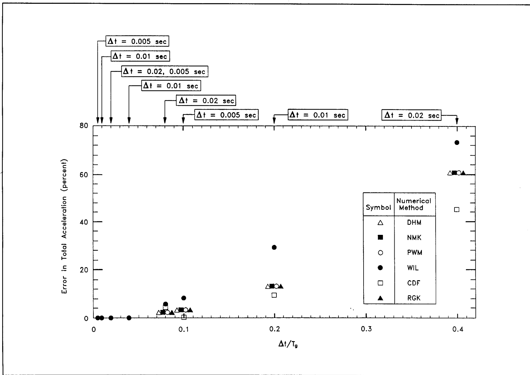
Figure 20. Percentile errors in maximum total acceleration (peak or valley value) for SDOF system of T_0 = 0.5 sec
