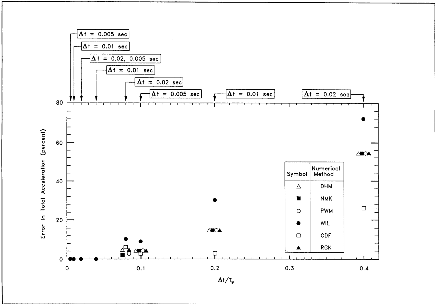
Figure 16. Percentile errors in maximum total acceleration (peak or valley value) for SDOF system of T_0 = 0.25 sec
