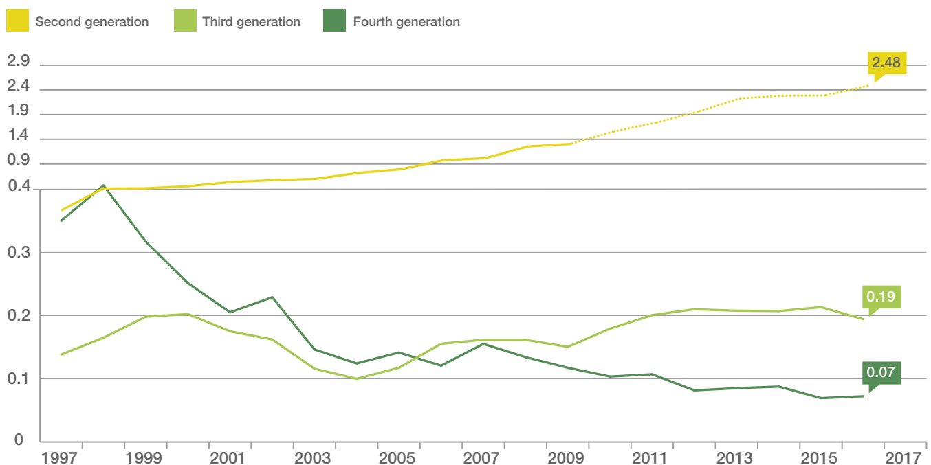
10 year moving average RE rate by aircraft generation per million flights
