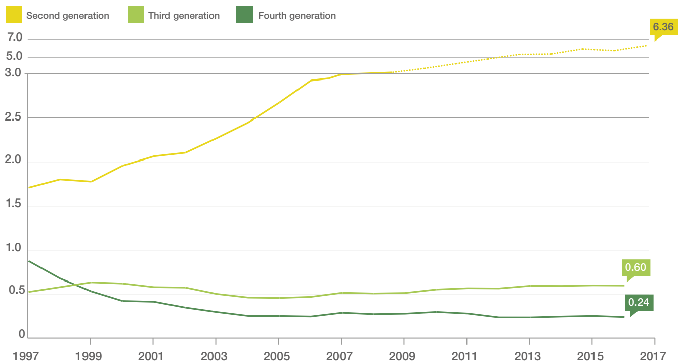
10 year moving average hull loss accident rate by aircraft generation per million flights 1997-2016
