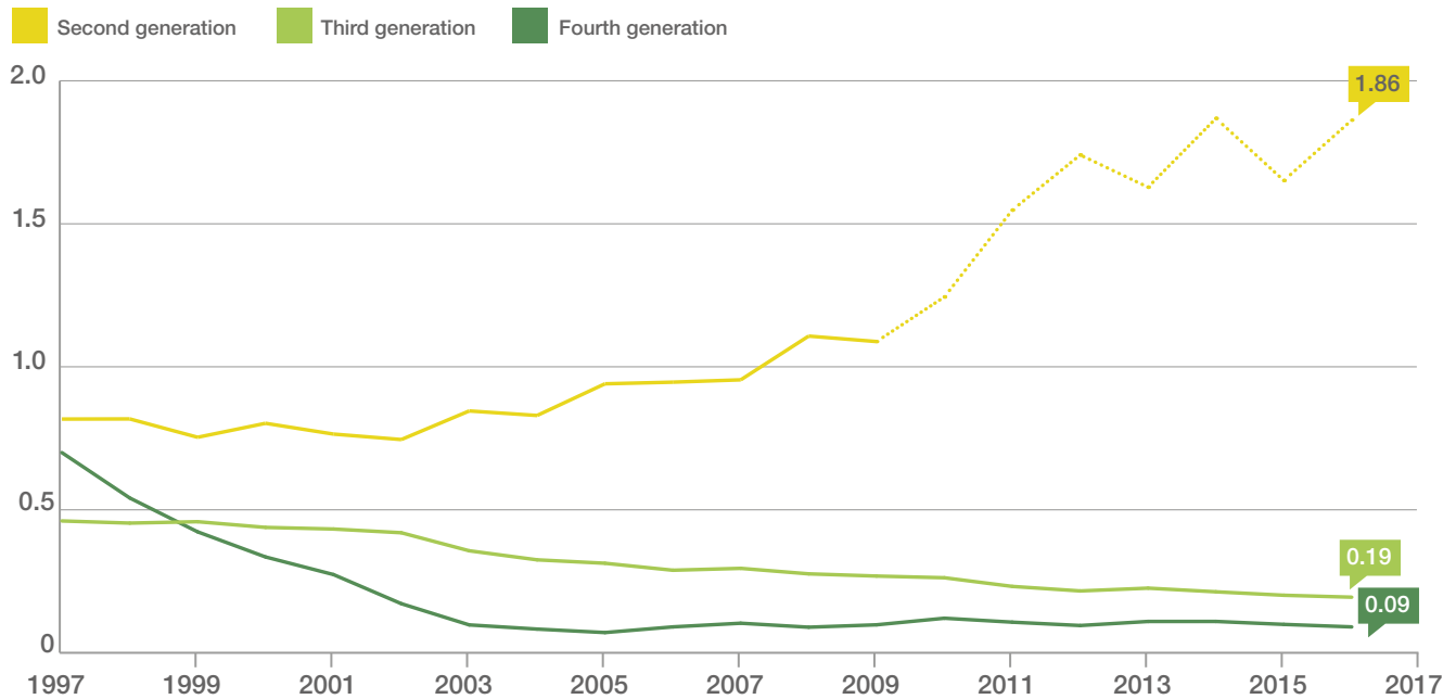
10 year moving average fatal accident rate by aircraft generation per million flights 1997-2016
