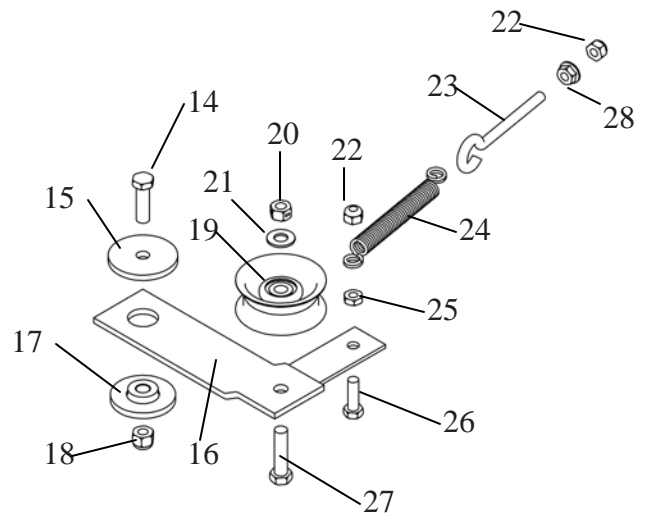
DETAIL 13
